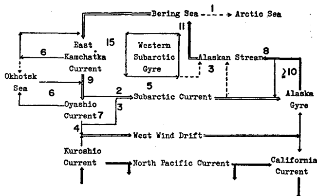
Fig. 3. Schematic diagram of relative transport in the northern North Pacific Ocean in winter. Numerals indicate volume transport ( \times 10^6 m 3 /sec) in reference to the 1,000-m. level.
