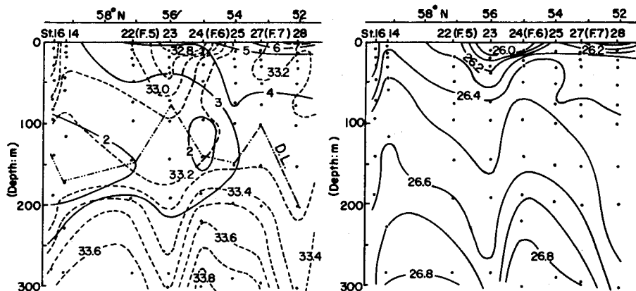
Fig. IV-13. Vertical sections of temperature ( ^{\circ}\text{C} ), salinity ( \text{‰} ) and sigma-t along long. 179^{\circ}\text{W} in the Bering Sea in early June, 1965.
