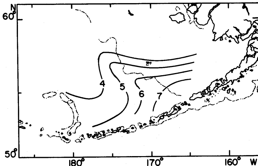
Fig. IV-25. Distribution of mean temperature ( ^{\circ}\text{C} ) at 20 meters in the eastern Bering Sea, June-July, 1962-1967.
