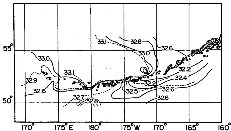
Fig. II-10. Distribution of salinity ( \text{‰} ) at 10 meters near the Aleutian Islands. (Dodimead, 1958)
