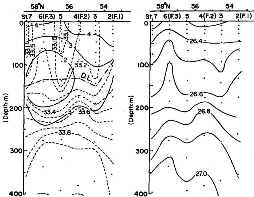
Fig. IV-15. Vertical sections of temperature ( ^{\circ}\text{C} ), salinity ( \text{‰} ) and sigma-t along long. 177^{\circ}\text{E} in the Bering Sea in middle June, 1966.
