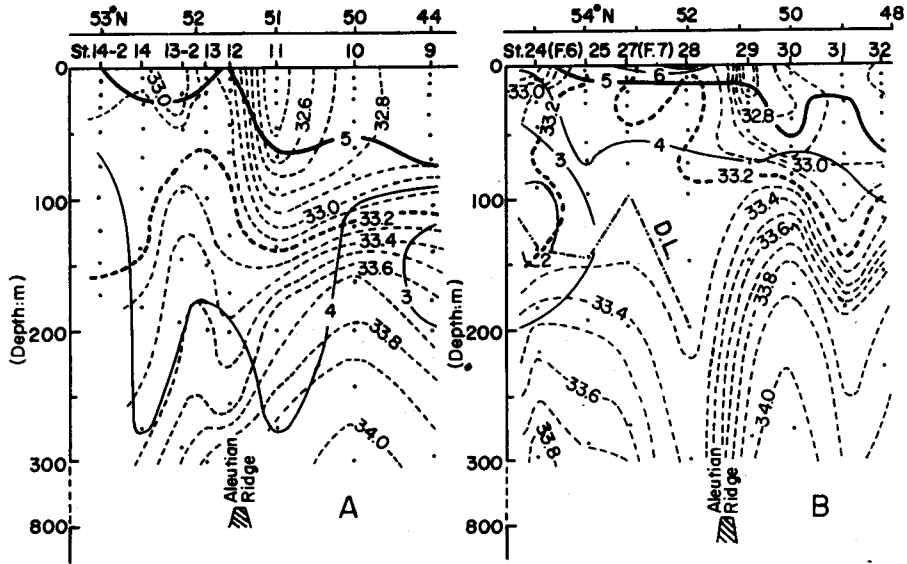
Fig. IV-6-A. Vertical sections of temperature (°C) and salinity (‰) of Amchitka Pass of the normal type (A), and soon after sockeye salmon have passed (B) in Amchitka Pass, in middle June.
