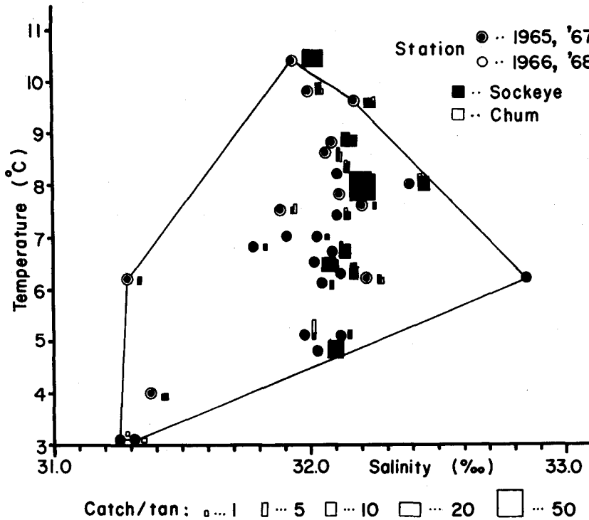
Fig. V-7. Relation between catch of sockeye salmon and temperature and salinity in the Bristol Bay area.
