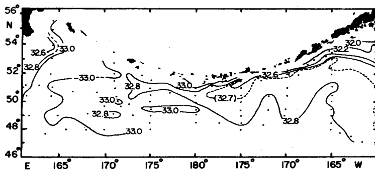
Fig. II-4. Distribution of surface salinity (‰), summer 1959. (Favorite, 1967)
