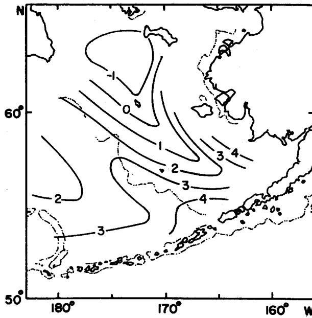
Fig. IV-27. Distribution of mean temperature ( ^{\circ}\text{C} ) in the dichothermal layer over the basin and sea bottom over the continental shelf in the eastern Bering Sea, June-July, 1962-1967.
