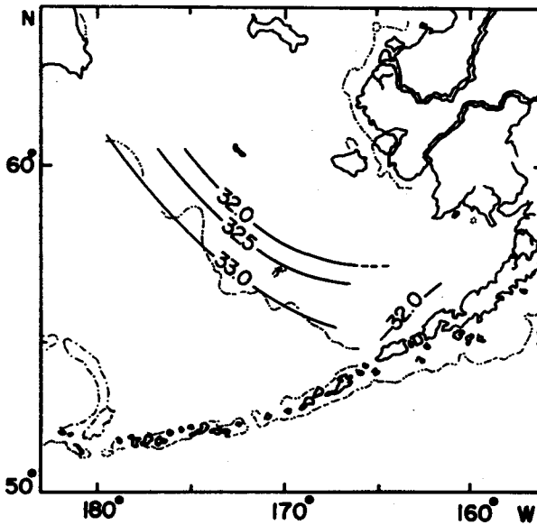
Fig. IV-28. Distribution of mean salinity ( \text{‰} ) in the dichothermal layer over the basin and sea bottom over the continental shelf in the eastern Bering Sea, June-July, 1962-1967.
