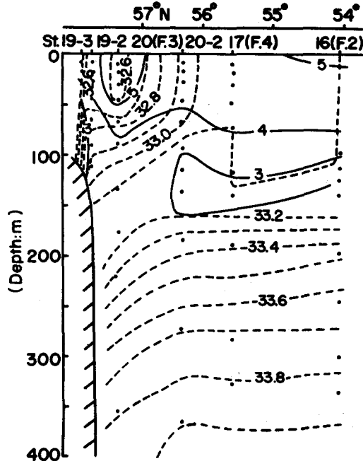
Fig. IV-21. Vertical sections of temperature ( ^{\circ}\text{C} ) and salinity ( \text{‰} ) from Amchitka Pass north-northeast to the continental slope in middle June, 1963.
