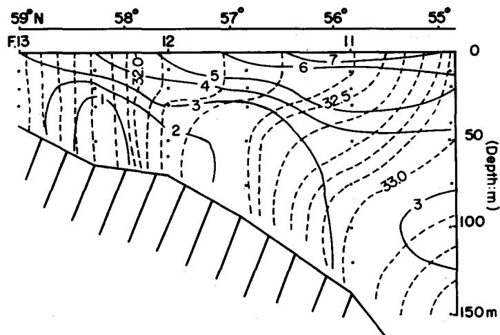
Fig. IV-30-A. Vertical sections of temperature (°C) and salinity (‰), and exploratory fishing stations along long. 168°W in late June, 1966.
