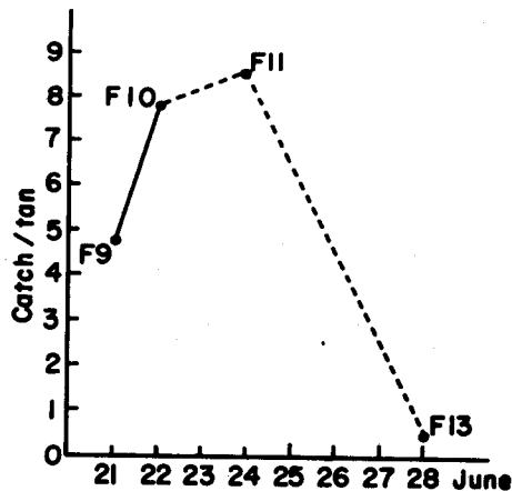
Fig. IV-24. The change of catch of sockeye salmon at the same position (54.9°N, 169.4°W) over the continental slope of the southeastern Bering Sea, June 1964.
