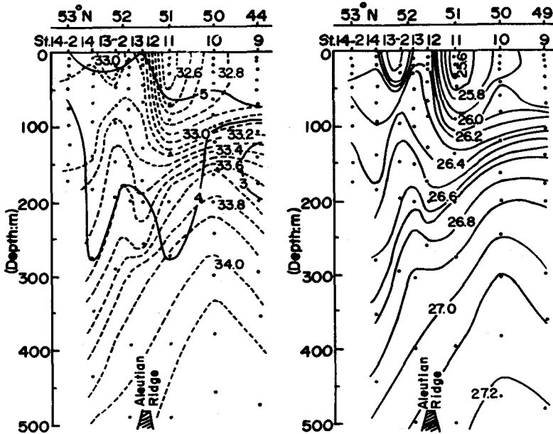
Fig. IV-1. Vertical sections of temperature (°C), salinity (‰) and sigma-t at Amchitka Pass (about longitude 179°W) in middle June, 1963.
