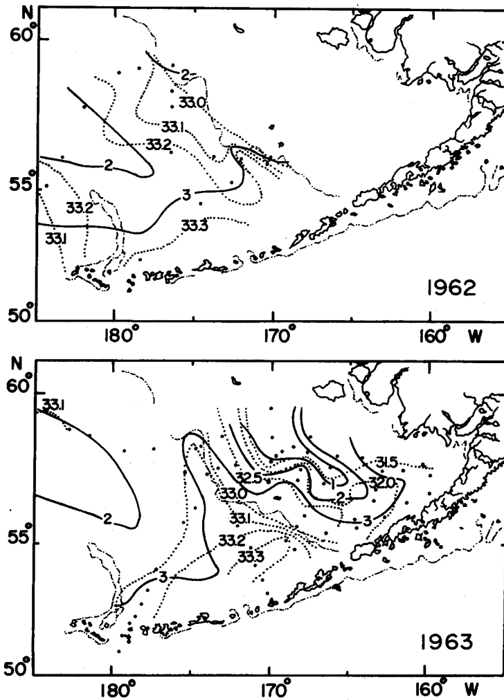
Fig. IV-8. Distribution of temperature ( ^{\circ}\text{C} ) and salinity ( \text{‰} ) in the dichothermal layer over the basin and sea bottom over the continental shelf in the eastern Bering Sea from June to July in each year, 1962-1967.
