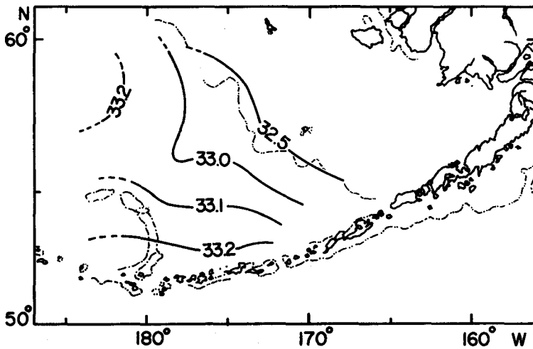
Fig. IV-10. Distribution of mean salinity (‰) at 20 meters over the basin in the eastern Bering Sea in June, 1962-1967.
