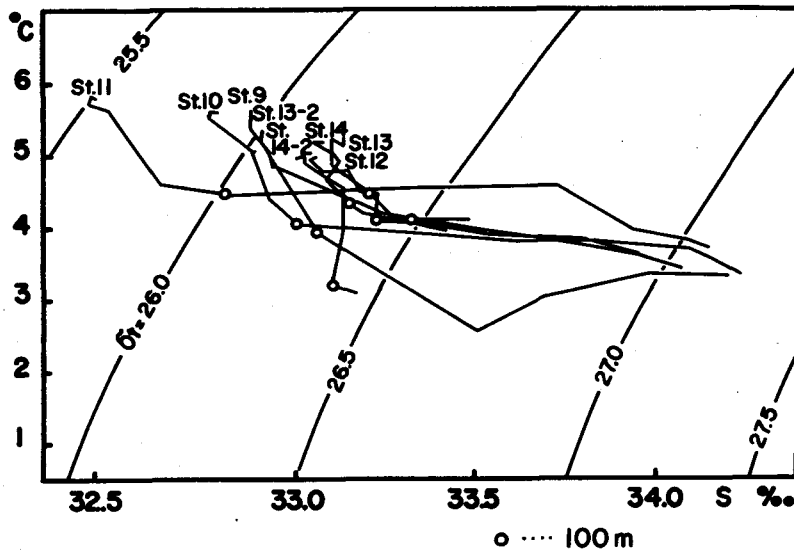
Fig. IV-5. T-S diagram at stations in Amchitka Pass in middle June, 1963.
