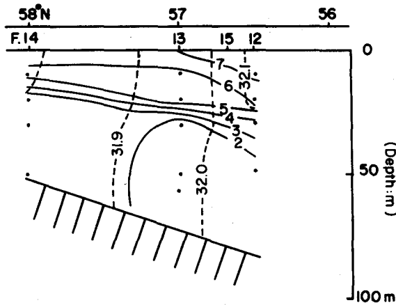
Fig. IV-32-B. Vertical sections of temperature ( ^{\circ}\text{C} ) and salinity ( \text{‰} ), and exploratory fishing stations along long. 165^{\circ}\text{W} in early July, 1968.
