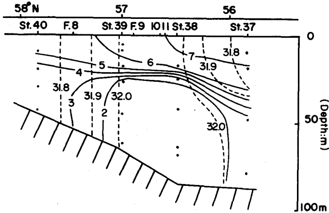
Fig. IV-32-A. Vertical sections of temperature ( ^{\circ}\text{C} ) and salinity ( \text{‰} ), and exploratory fishing stations along long. 163^{\circ}\text{W} in late June, 1968.
