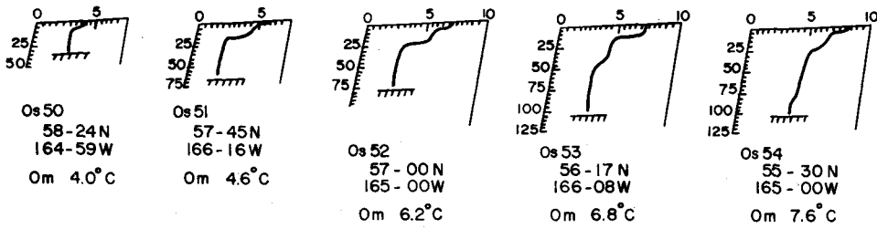
Fig. IV-33. B-T records along longitude 165°W in late June, 1965.
