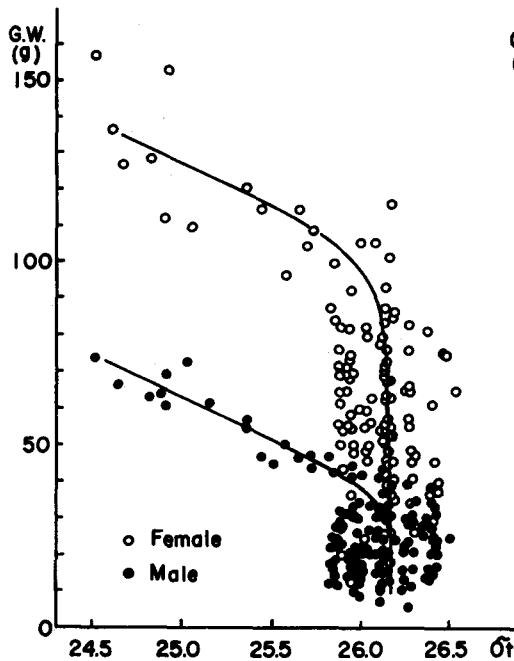
Fig. V-9. Relation between gonad weight of mature sockeye salmon in 5 s age and sigma-t in the area from south of the Aleutian Islands to Bristol Bay, through the eastern Bering Sea.
