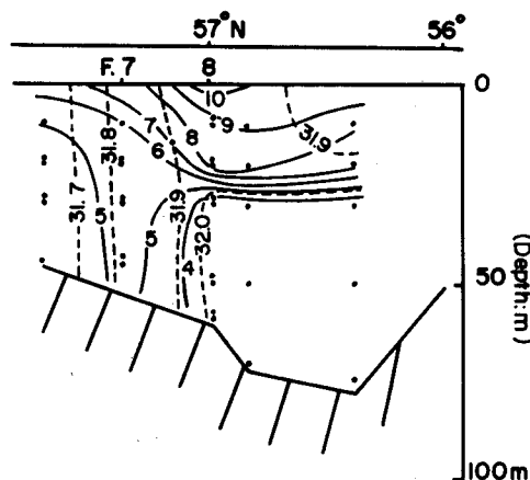
Fig. IV-31-A. Vertical sections of temperature (°C) and salinity (‰), and exploratory fishing stations along long. 162°W in late June, 1967.
