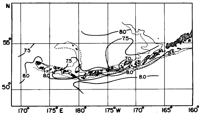
Fig. II-9. Distribution of temperature ( ^{\circ}\text{C} ) at 10 meters near the Aleutian Islands. (Dodimead, 1958)
