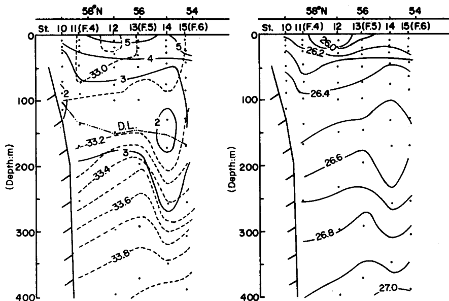
Fig. IV-14. Vertical sections of temperature ( ^{\circ}\text{C} ), salinity ( \text{‰} ) and sigma-t along long. 176^{\circ}\text{W} in the Bering Sea in middle June, 1966.
