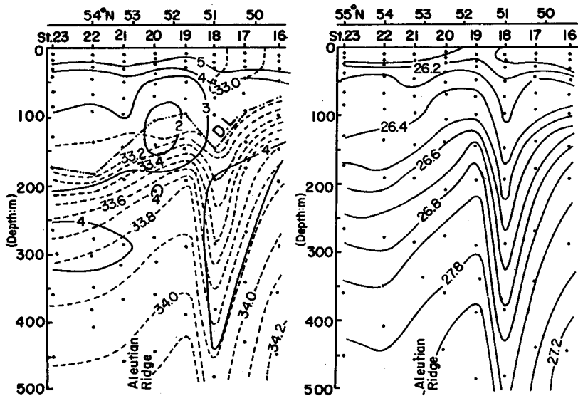
Fig. IV-3. Vertical sections of temperature ( ^{\circ}\text{C} ), salinity ( \text{‰} ) and sigma-t at the Pass along long. 173^{\circ}\text{E} in late June, 1964.
