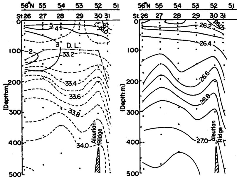
Fig. IV-2. Vertical sections of temperature ( ^{\circ}\text{C} ), salinity ( \text{‰} ) and sigma-t at the Pass along 175^{\circ}\text{E} in late June, 1964.
