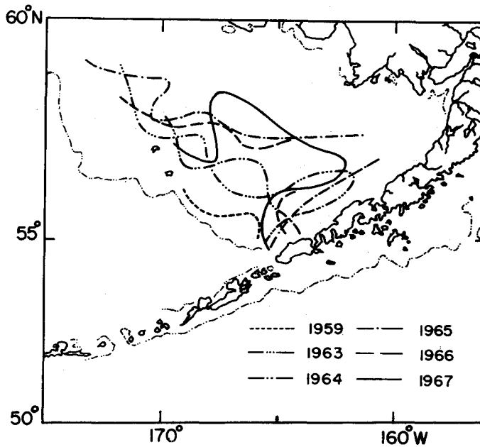
Fig. IV-34. Distribution of the 32.0‰ isohaline at 20 meters in outer Bristol Bay, June to early July in each year, 1959 and 1963-1967.
