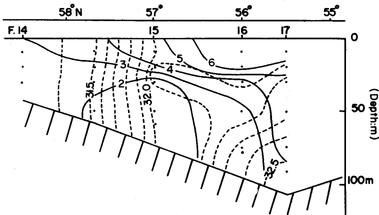
Fig. IV-30-B. Vertical sections of temperature ( ^{\circ}\text{C} ) and salinity ( \text{‰} ), and exploratory fishing stations along long. 165^{\circ}\text{W} in late June, 1966.
