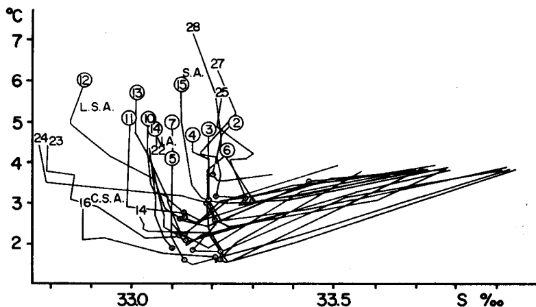
Fig. IV-17. T-S diagram of continental slope stations in the eastern Bering Sea, 1965 and 1966.
