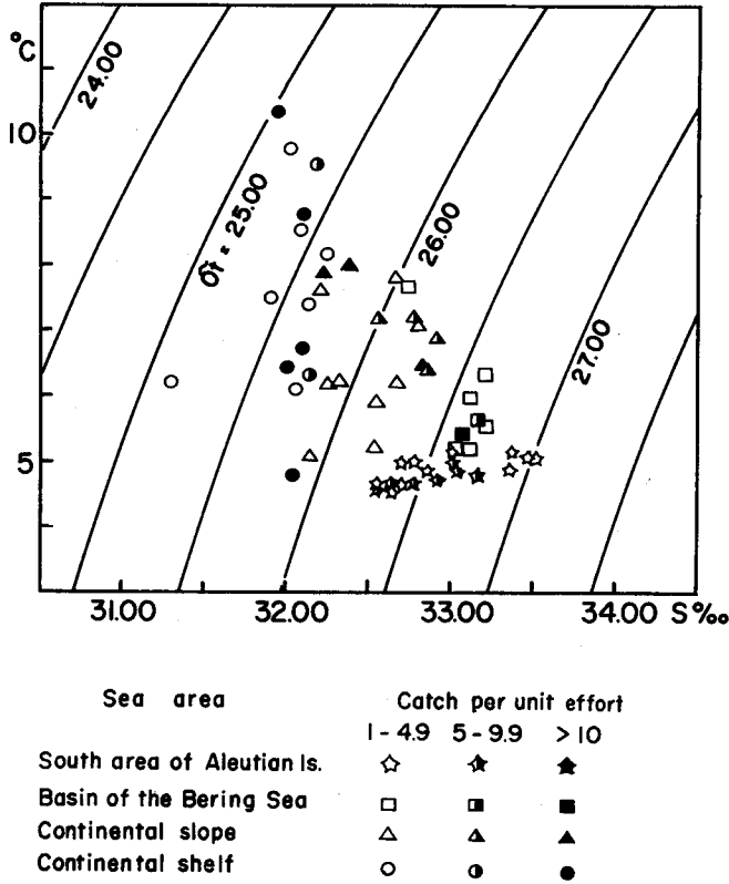
Fig. V-8. Relation between the catch of sockeye salmon and temperature-salinity (T-S diagram) at stations occupied in areas from south of the Aleutian Islands to Bristol Bay through the eastern Bering Sea.
