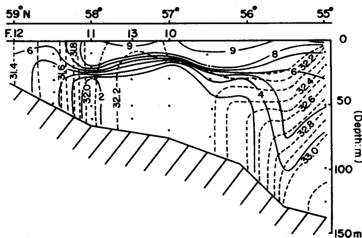
Fig. IV-31-B. Vertical sections of temperature (°C) and salinity (‰), and exploratory fishing stations along long. 166°W in late June, 1967.
