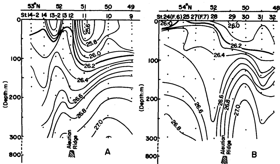
Fig. IV-6-B. Vertical sections of sigma-t of Amchitka Pass of the normal type (A), and after sockeye salmon have passed through (B) in middle June.
