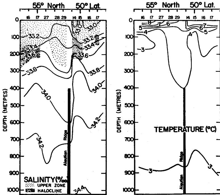
Fig. II-8-B. Vertical section of salinity and temperature along long. 180°, summer, 1957. (Dodimead et al., 1963)
