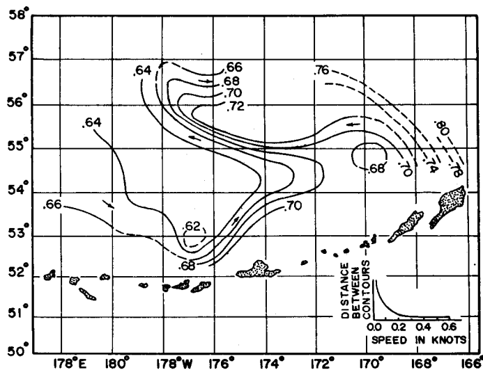
Fig. II-12. Dynamic height anomaly, 0/500 db. Bering Sea, July-August 1949. (Saur et al., 1952)
