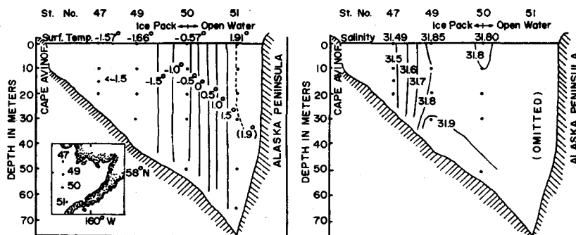
Fig. II-14. Vertical sections of temperature ( ^{\circ}\text{C} ) and salinity ( \text{‰} ) at the mouth of the Bristol Bay in winter, 1955. (U.S. Navy Hydrographic Office, 1958)
