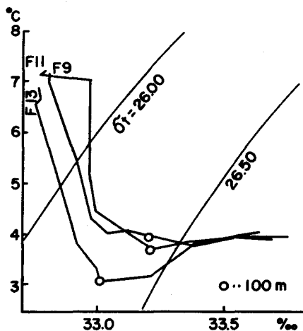
Fig. V-6. T-S diagrams at the same position (54.9°N, 169.4°W) on the continental slope of the southeastern Bering Sea, 1964.
