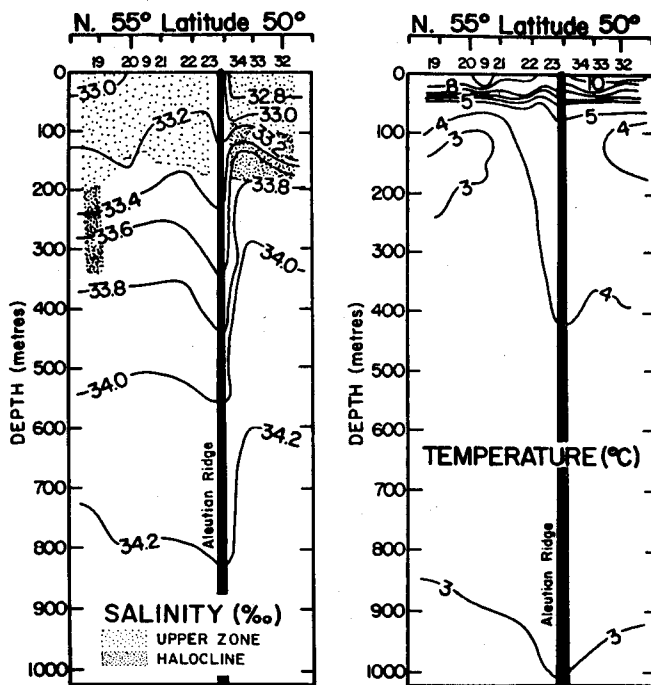
Fig. II-8-C. Vertical section of salinity and temperature along long. 175°W, summer, 1957. (Dodimead et al., 1963)
