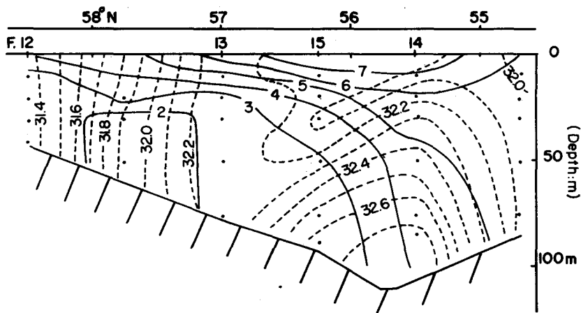
Fig. IV-29. Vertical sections of temperature (°C) and salinity (‰), and exploratory fishing stations along long. 165°W in late June, 1965.
