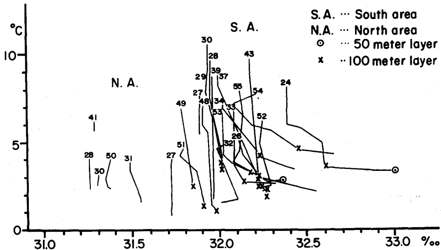
Fig. IV-35. T-S diagram from stations in Bristol Bay, 1965-1968.
