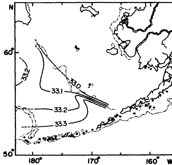
Fig. IV-12. Distribution of mean salinity ( \text{‰} ) in dichothermal layer over the basin in the eastern Bering Sea in June, 1962-1967.
