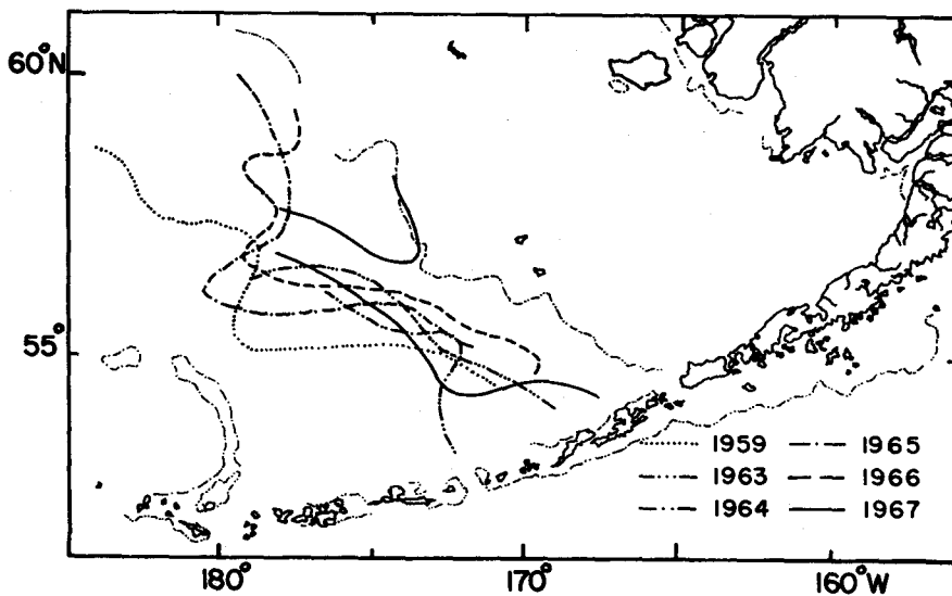
Fig. IV-16. Distribution of 33.0\text{‰} isohaline at 20 meters in the eastern Bering Sea, from June to July, 1959 and 1963-1967.
