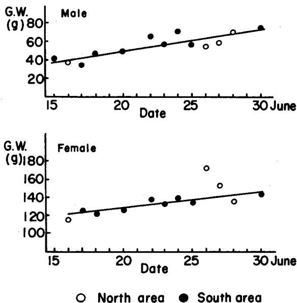
Fig. V-11. Time change of mean gonad weight of the 6 + age group of western Alaska sockeye salmon during migration in the eastern Bering Sea, middle to late June, 1966.
