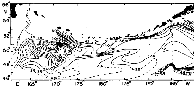
Fig. II-3. Distribution of temperature (°C) in the temperature-minimum stratum, summer 1959. (Favorite, 1967)
