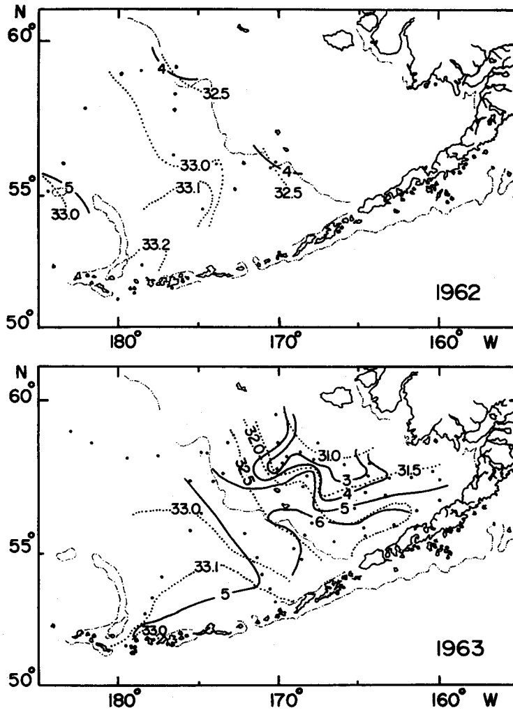
Fig. IV-7. Distribution of temperature ( ^{\circ}\text{C} ) and salinity ( \text{‰} ) at 20 meters in the eastern Bering Sea from June to July in each year, 1962-1967.
