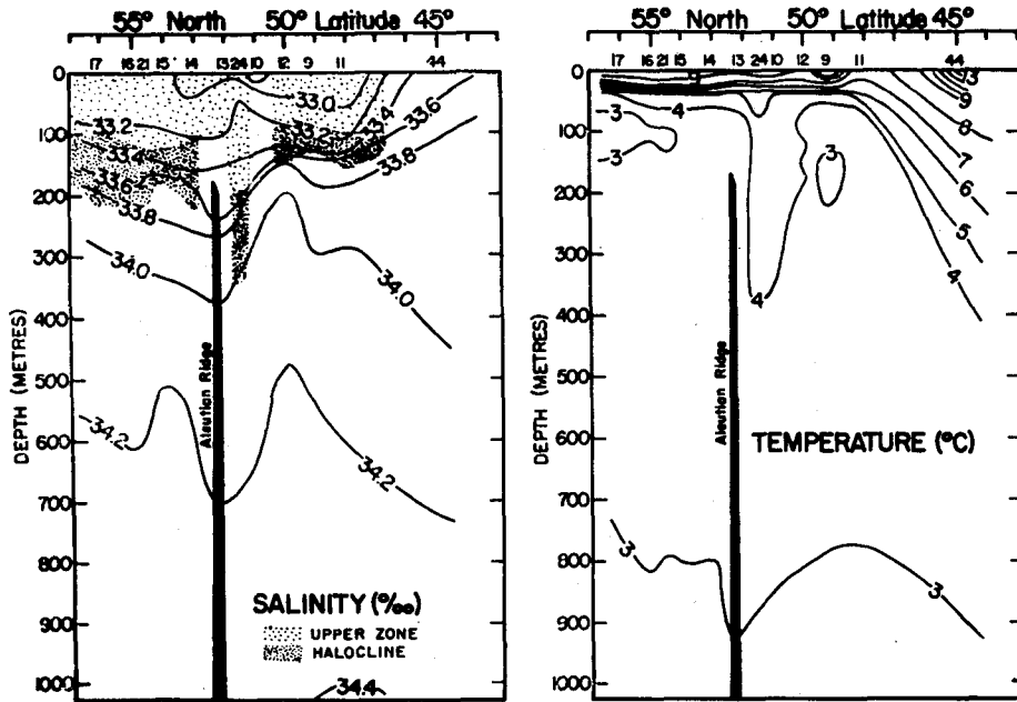
Fig. II-8-A. Vertical section of salinity and temperature along long. 175°E, summer, 1957. (Dodimead et al., 1963)
