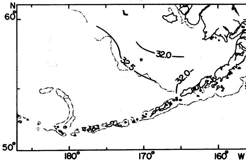
Fig. IV-26. Distribution of mean salinity ( \text{‰} ) at 20 meters in the eastern Bering Sea, June-July, 1962-1967.
