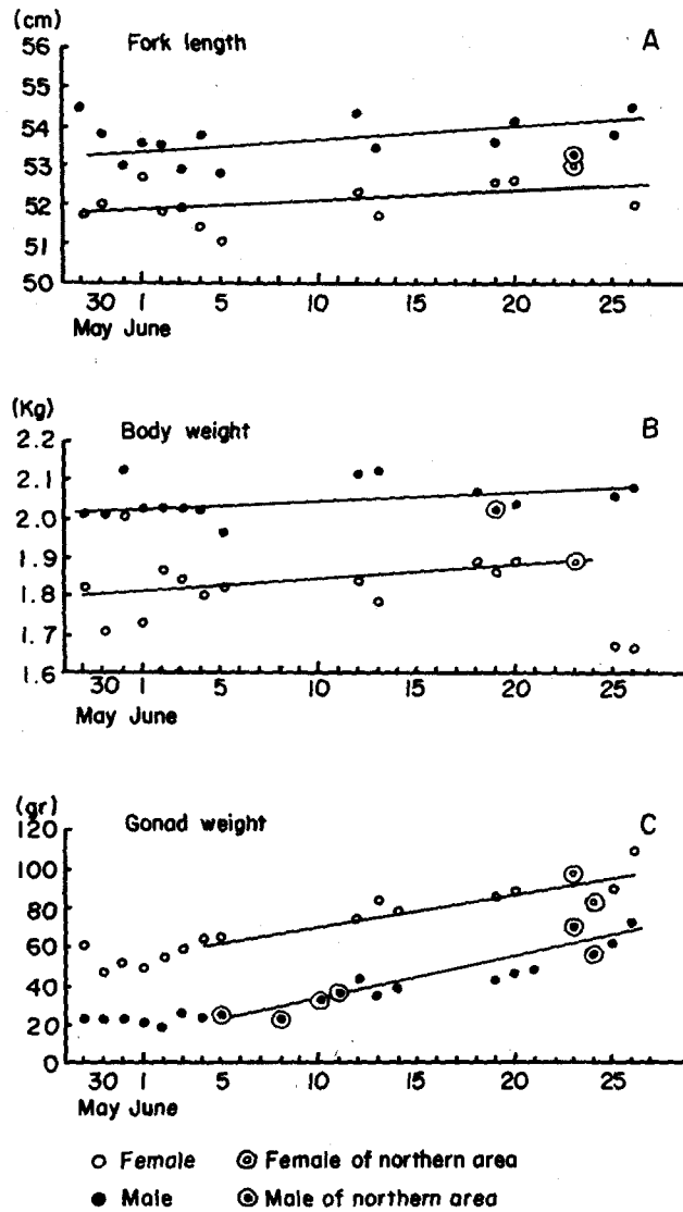
Fig. V-3. Changes of mean fork length (A), body weight (B) and gonad weight (C) with time of the 5, age group of western Alaska sockeye salmon during migration from the southern area of Aleutian Islands to Bristol Bay in early summer, 1965.
