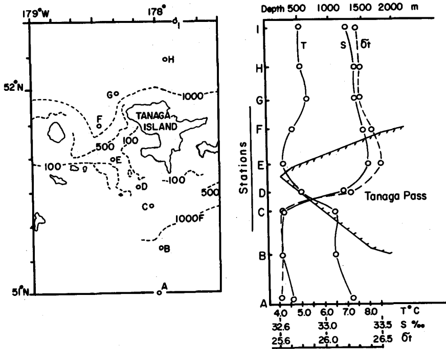
Fig. IV-4. Distribution of stations (left) and the surface distribution of temperature (°C), salinity (‰) and sigma-t (right) in Tanaga Pass, in middle June, 1967.
