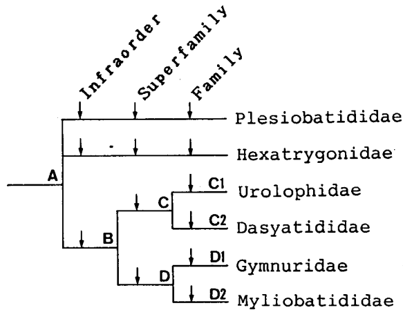
Fig. 73. Phylogenetic classification. Ranking of higher taxonomic levels.
