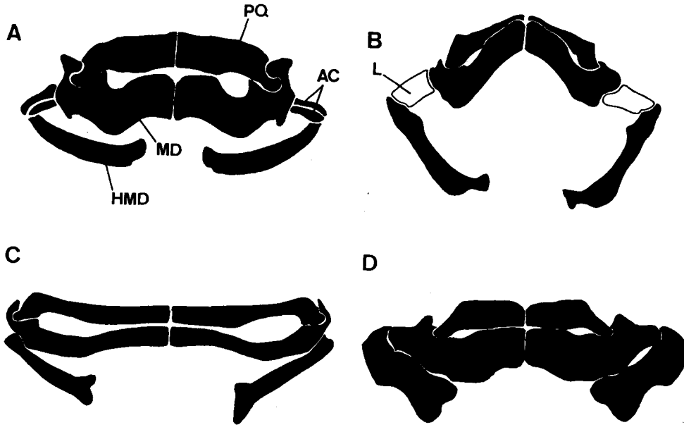
Fig. 24. Ventral view of the hyomandibular-mandibular articulation. A, Potamotrygon yepezi ; B, Dasyatis pastinaca ; C, Aetoplatea zonura ; D, Narke japonica . AC, angular cartilage; HMD, hyomandibular cartilage; L, ligament; MD, mandibular cartilage; PQ, palatoquadrate cartilage.
