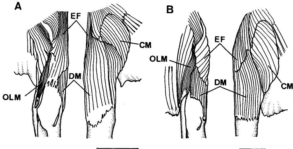
Fig. 61. Dorsal (left) and ventral (right) views of the clasper muscles in two myliobatidoids. A, Potamotrygon yepezi ; B, Myliobatis goodiei . CM, compressor muscle; DM, dilatator muscle; EF, external flexor; OLM, outer lip muscle. Scales indicate 10 mm.
