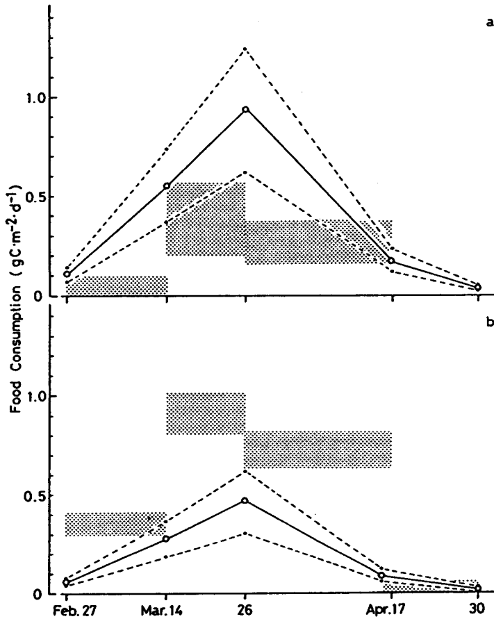
Fig. 24. Temporal changes in the food consumption by phagotrophic dinoflagellates within the upper 30 m. Calculations are conducted using the mean clearance rate (Lessard and Swift, 1985) (open circles and solid lines). 95% confidence limits of clearance rate are also used (closed circles and broken lines). Different sets of carbon to chlorophyll a ratio are used, i.e., (a) 50 during February and March, 120 during April, (b) 25 during the former period and 60 during the latter. Dotted area denotes the shortage in food consumption by the total zooplankters except phagotrophic dinoflagellates to grazed carbon calculated by equation 8.
