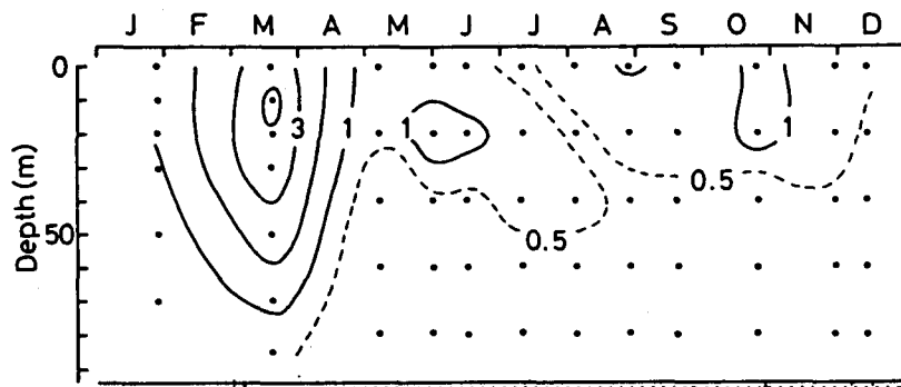
Fig. 8. Vertical profile of chlorophyll a concentration ( \mu\text{g}\cdot\text{L}^{-1} ) observed at Station 30 in 1988.
