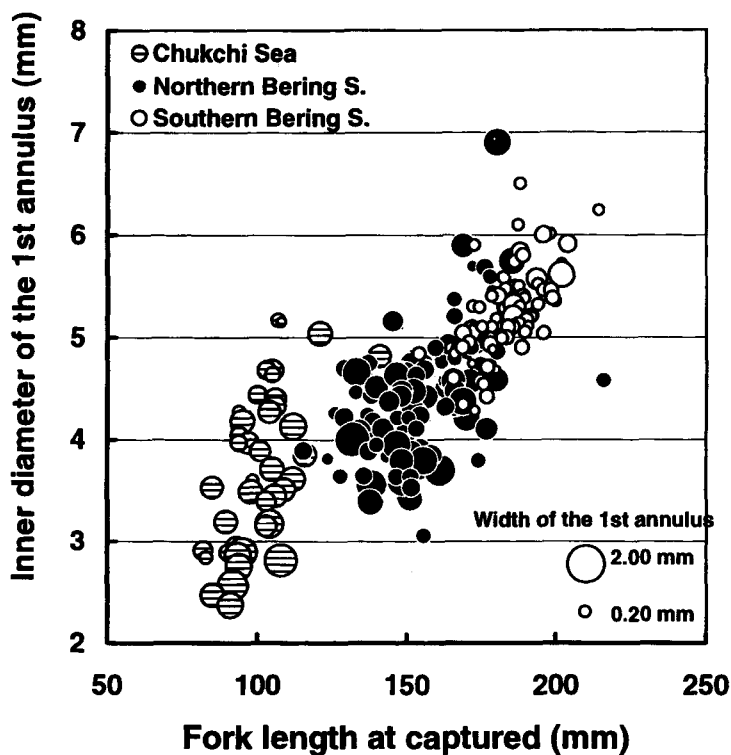
Fig. 2. Relationship between fork length at capture and inner diameter of the 1st annulus in the otolith of age 1 walleye pollock. Radius of each bubble represents the width of the 1st annulus.
