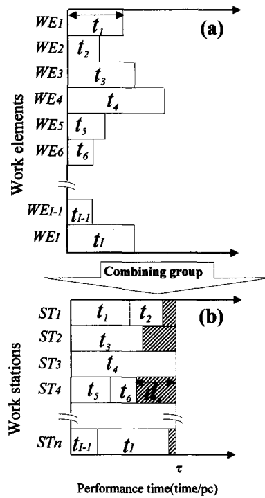
Fig. 14. Schematic diagrams of (a) the original and (b) combined work elements. t_i is the standard time of the i -th work element ( i=1, 2, 3, \dots, I ). d_k and \tau show the idle time of the k -th work station ( k=1, 2, 3, \dots, n; n \leq I ) and cycle time respectively. The hatched area is the sum of idle time in the line production system. The unit of performance time (time/pc) is the necessary for processing one of item.
