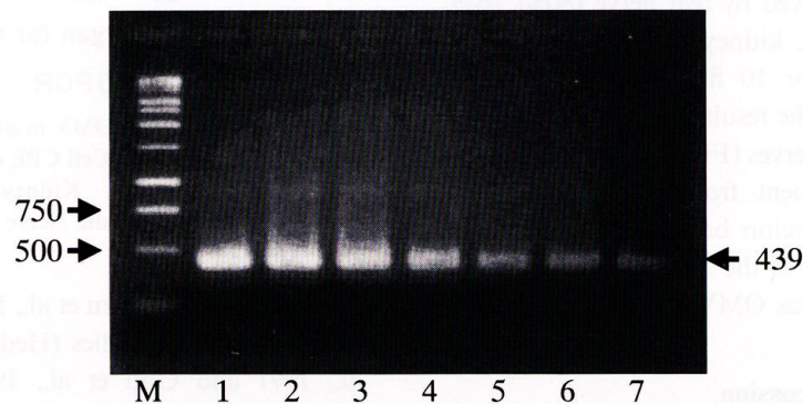
Fig. 2. Agarose gel electrophoresis of PCR amplification products from diluted virus suspension of OMV 00-7812. Gel was stained with EtBr. Lanes : M ; DNA molecular weight marker, 1 ; OMV 00-7812 strain, 2 ; 10^{5.8} TCID 50 /ml, 3 ; 10^{4.8} TCID 50 /ml, 4 ; 10^{3.8} TCID 50 /ml, 5 ; 10^{2.8} TCID 50 /ml, 6 ; 10^{1.8} TCID 50 /ml, 7 ; 10^{0.8} TCID 50 /ml.
