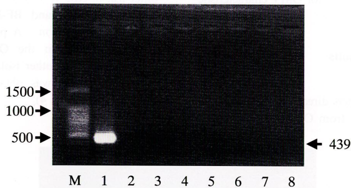
Fig. 4. Agarose gel electrophoresis of PCR amplification products from seven other fish disease viruses. Gel was stained with EtBr. Lanes: M; DNA molecular weight marker, 1; OMV 00-7812, 2; IHNV, 3; IPNV, 4; HIRRV, 5; SRV, 6; RSIV, 7; JF-LCDV, 8; BF-NNV.
