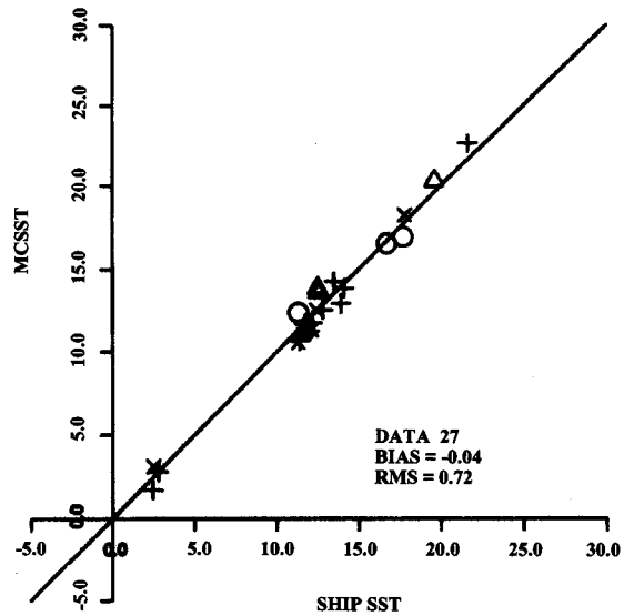
Fig. 2. The comparison between MCSST and Ship-SST. Each symbol shows the difference of observation times between satellite and ship, + shows within 1 h, × shows within 2 h, Δ shows within 3 h and ○ shows within 4 h.
