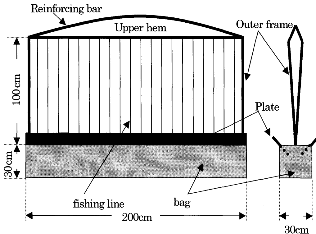
Fig. 1. Sketch of harp trap of squarely view (1) and profile view (2).
