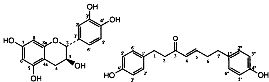
(2) plataphyllenone
