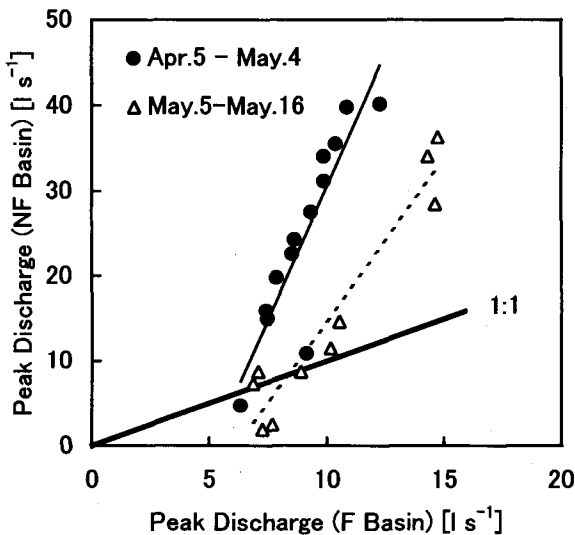
Fig.7. Comparison of peak discharges for snowmelt between the F and NF basin. Solid line and broken line mean the trend for early and late periods respectively.
