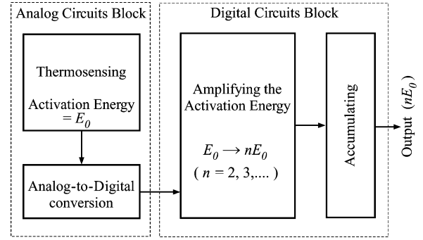
Fig. 1. Construction of our sensor device.
