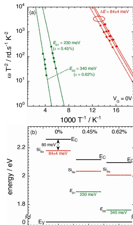
FIG. 7. (Color online) (a) Thermal emission rate related to each conductance peak as a function of reciprocal temperature and (b) the energy position of the levels detected in the Ni/GaP 1-x N x ( x=0\% , 0.45%, and 0.62%) alloys.
