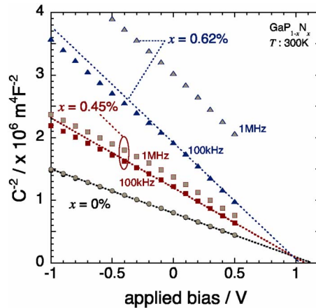
FIG. 5. (Color online) C^{-2} - V characteristics of Ni/Au Schottky contacts on the GaP 1-x N x surfaces at RT. The circle, rectangle, and triangle shapes represent the result of x=0\% , 0.45\% , and 0.62\% , respectively. The circles, rectangles, and triangles represent the results for x=0\% , 0.45\% , and 0.62\% , respectively.
