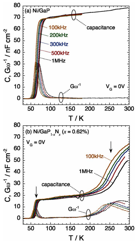
FIG. 6. (Color online) Typical thermal admittance spectra taken from the (a) Ni/GaP and (b) Ni/GaP 1-x N x ( x=0.62\% ) interface at a temperature ranging from 30 to 300 K. The measurement was done at a frequency of 1 MHz, 500 kHz, 300 kHz, 200 kHz, and 100 kHz, respectively, with an ac signal rms value of 20 mV.
