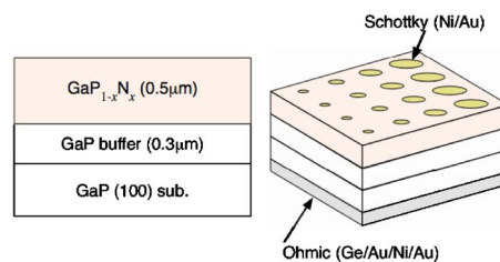
FIG. 1. (Color online) Schematic representation of the GaPN layered structure and the fabricated Schottky diode structure.
