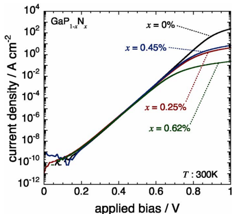
FIG. 4. (Color online) Typical forward I - V characteristics of a Ni/Au Schottky contact on the GaP 1-x N x ( x=0, 0.25, 0.45, and 0.62\% ) surfaces at RT.
