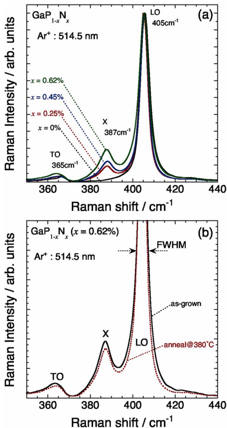
FIG. 3. (Color online) (a) Typical resonant Raman scattering spectra of the GaP alloys measured at RT and (b) the spectra of the GaP 1-x N x ( x=0.62\% ) alloy before and after annealing at 380 °C. The spectra obtained were normalized by the intensity of the LO line.
