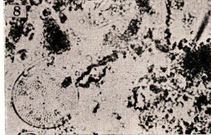
(C) Biological Constituents of Marine Snow . Kagoshima Bay \times 360 Surface water
