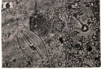
(C) Biological Constituents of Marine Snow . Kagoshima Bay \times 360 Surface water
