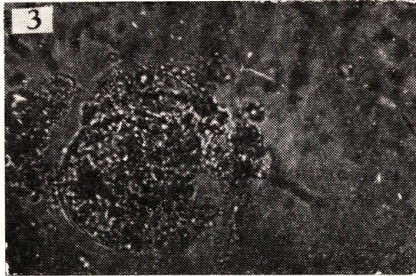
(B) Some Stages in Disintegration Process of Diatom, Coscinodiscus sp. Mutsu Bay \times 360
