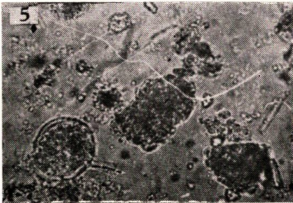
(C) Biological Constituents of Marine Snow . Kagoshima Bay \times 360 Surface water
