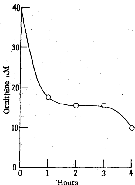
Fig. 5. Changes of rate of ornithine disappearance during the incubation of ornithine with cells adapted with arginine
