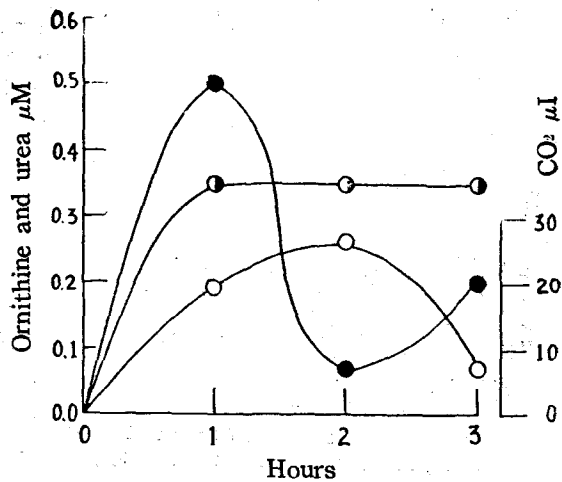
Fig. 2. Changes during the incubation of arginine with washed cell suspensions of Bac. subtilis
