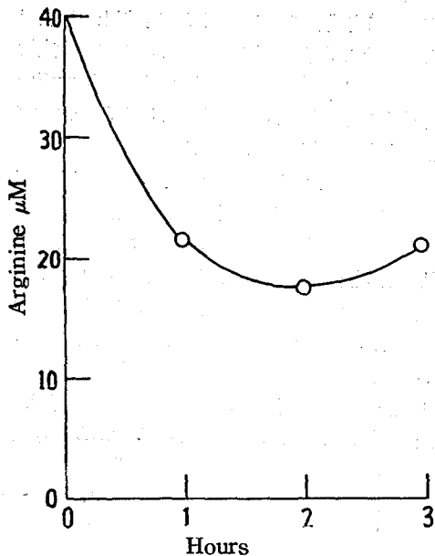
Fig. 1. Changes of rate of arginine disappearance during the incubation of arginine with washed cell suspensions of Bac. subtilis
