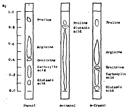
Fig. 3. Paper chromatograms of reaction mixtures Run in phenol (contained 23 per cent of water), methanol (methanol:water=8:2), m-cresol (contained 25 per cent of water). Sprayed with ninhydrin-butanol solution.
