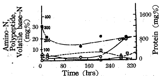
Fig. 6. Changes in the amounts of several fractionated nitrogens in alkali solution (pH 8.9)
