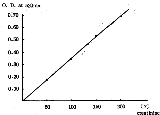
Fig. 2. Relationship between the concentration of creatinine and extinction (Spectrophotometer)
