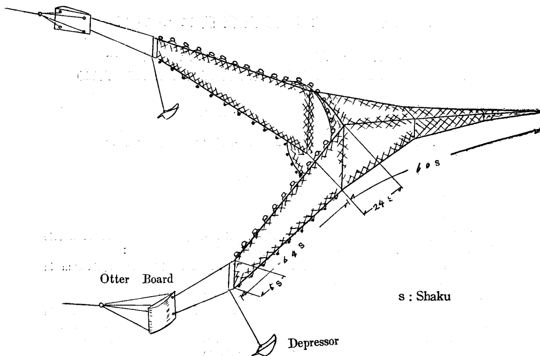
Fig. 1 Mid-water trawl gear
