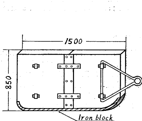
Fig. 2 Otter-board
