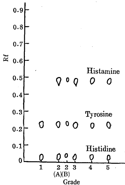
Fig. 1. Diazo reaction positive substances in dried squid meat graded into the first to the fifth
