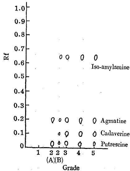
Fig. 2. Volatile bases in dried squid meat graded into the first to the fifth
