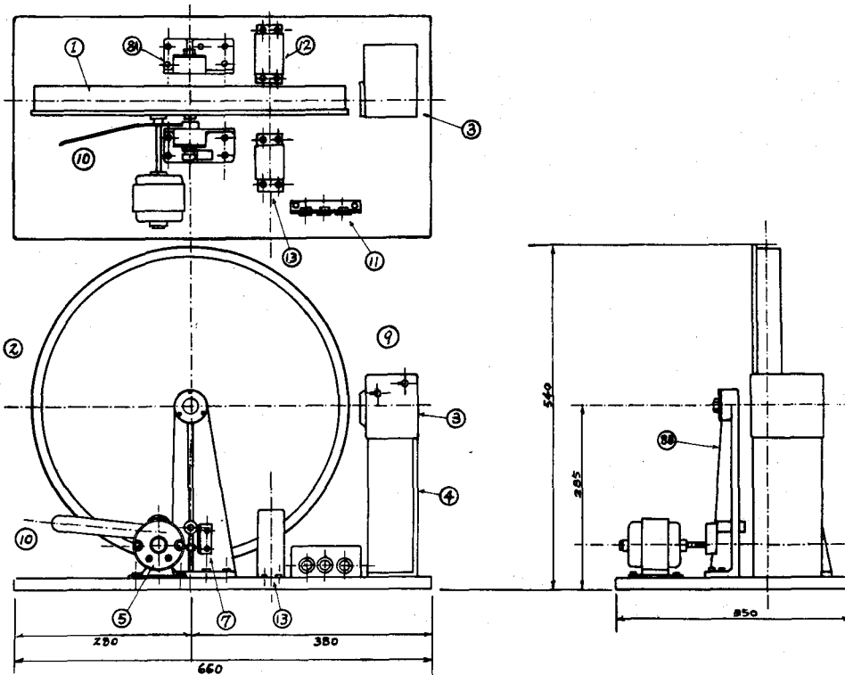
Fig. 2. Diagram of the mechanical part of the function and signal generator
