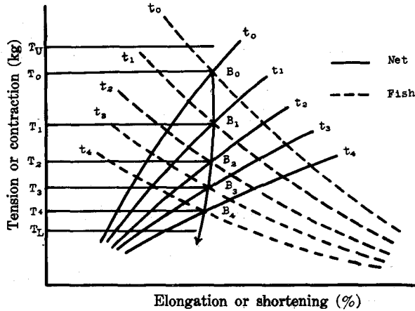
Fig. 4. Dynamical relationship tension (contraction) and elongation (shortening) under the sticking condition
