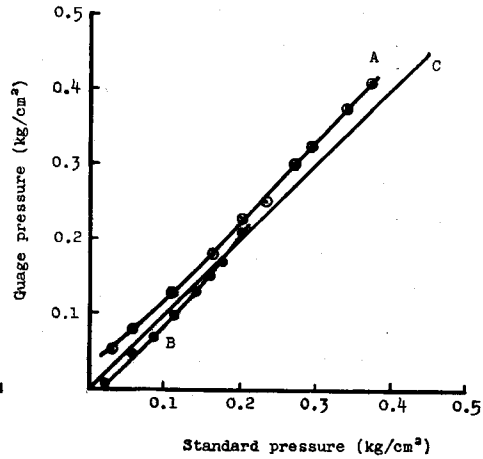
Fig. 9 Calibration curves of pressure gauges Standard pressure (abscissa) was measured by a manometer of mercury.
