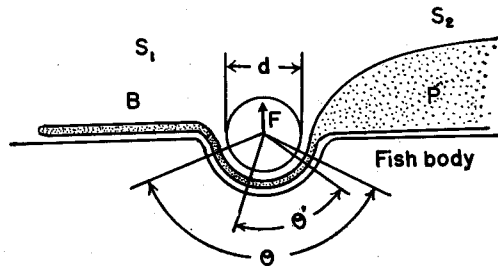
Fig. 6 Positional relationship between net-tension and bag-pressure when the vinyl membrane was inserted under the net twine on the surface of fish body
