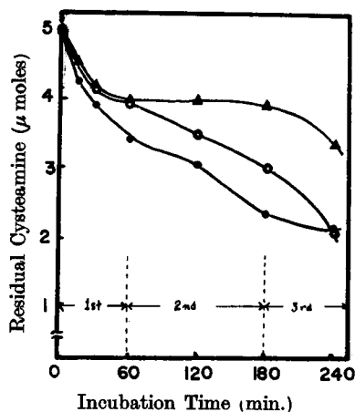
Fig. 4. Changes in cysteamine during incubation. The standard assay system contained 0.2 ml of enzyme solution of fresh ligament muscle (-o-o-); 0.05 \mu moles of methylene blue contained (-•-•-); 0.60 \mu moles of sodium sulfide contained (-▲-▲-).
