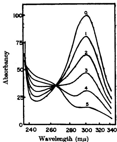
Fig. 1. Specific absorption and decrease of absorbancy at 300 mμ. with the addition of cysteine.
