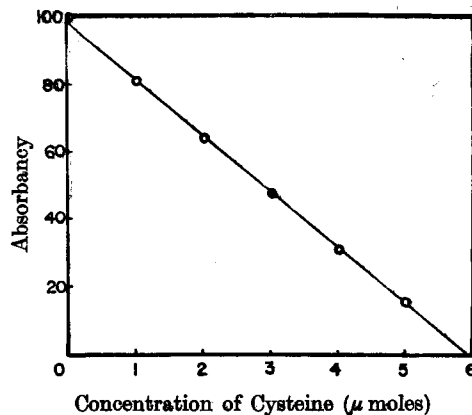
Fig. 2. Standard graph of cysteine. Decrease in absorbancy of NEM as a function of the amount of cysteine. Absorbancy: -\log T \times 10^3 at 300mμ. Medium: 0.25 M phosphate buffer pH 6.0.
