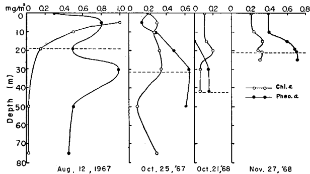
Fig. 3. Vertical distribution of chlorophyll a and pheophytin at Sta. 2 in Lake Toya. (...1% light intensity depth)
