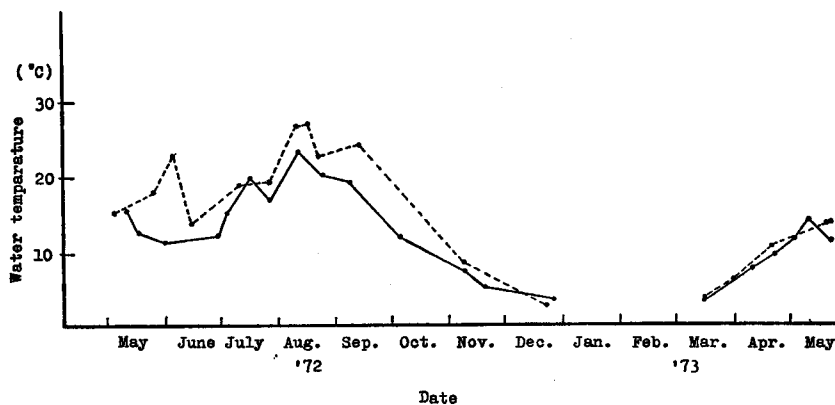
Text-fig. 3. Water temperature in the river Daitobetsu. ○ in the spawning area, ● in the upper course
