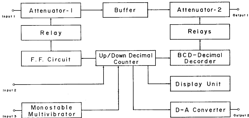
Fig. 4. Block diagram of the automatic attenuator.
