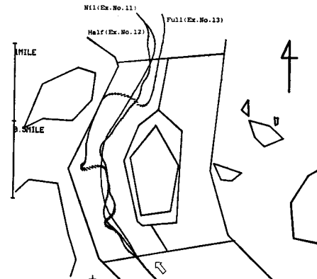
Fig. 36. Course-ultra-unstable ship's trajectories of northwardbound navigation by W3 deck officer in Nishi-Suido at nil (Ex. No. 11), half (Ex. No. 12) and full (Ex. No. 13) of the highest speed of tidal stream.
