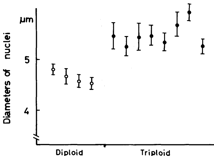
Text-Fig. 1. Nuclear size of the first spermatocyte of the diploid (○) and the triploid (●) crucian carp. Vertical bars indicate confidence limits at 99%.
