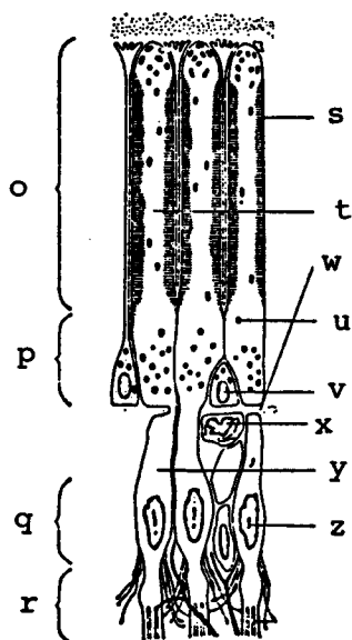
Fig. 2. Schematic representation of the structure of a cephalopod retina. [from Tazaki (1967) 8) ]. o: rhabdom layer, p: black pigment layer, q: layer of visual cell nucleus, r: layer of optic nerve fibers, s: rhabdomere, t: outer segment of visual cell, u: black pigment, v: support layer, w: limiting membrane, x: blood vessel, y: inner segment of visual cell, z: visual cell nucleus.
