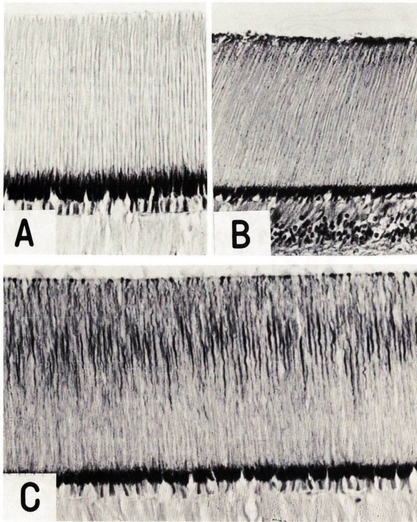
Fig. 3. Microphotographs showing the migrating condition of the black pigment in retina of the squids, Todarodes pacificus Steenstrup.
