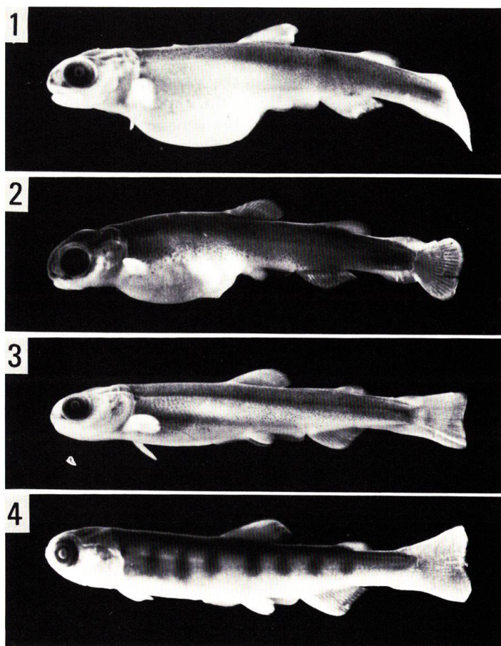
Fig. 1. The four types appeared in the hybrid fry of lot 3. 1: W-type, BL=27.5 mm; 2: S-type, BL=27.9 mm; 3: B-type, BL=31.1 mm; 4: N-type, BL=34.4 mm;
