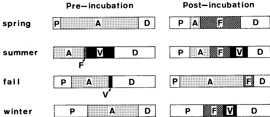
Fig. 5. Bacterial floras reducing the infectivity of IHNV in the water collected seasonally from 1984 to 1985 from the Nanaehama coast. Symbols: P, Pseudomonas ; A, Achromobacter ; F, Flavobacterium/Cytophaga ; V, Vibrio ; D, Dead and unidentified strains.
