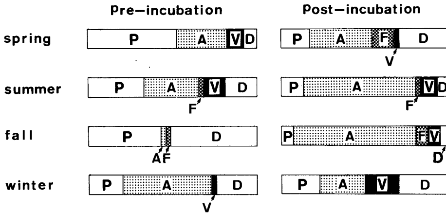
Fig. 6. Bacterial floras reducing the infectivity of IHNV in the sediment samples collected seasonally from 1984 to 1985 from the Nanaehama coast. Symbols: P, Pseudomonas ; A, Achromobacter ; F, Flavobacterium/Cytophaga ; V, Vibrio ; D, Dead and unidentified strains.
