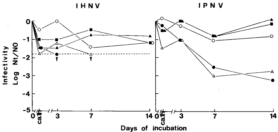
Fig. 2. Infectivities of fish pathogenic viruses in seawater and water-sediment mixture samples from the Nanaehama coast in August, 1984. Symbols: ■, autoclaved; ▲, filtered; ●, untreated; △, water-sediment mixture; ○, control. Dotted line and arrows indicate detectable limits of viral titres and less than the limits respectively.
