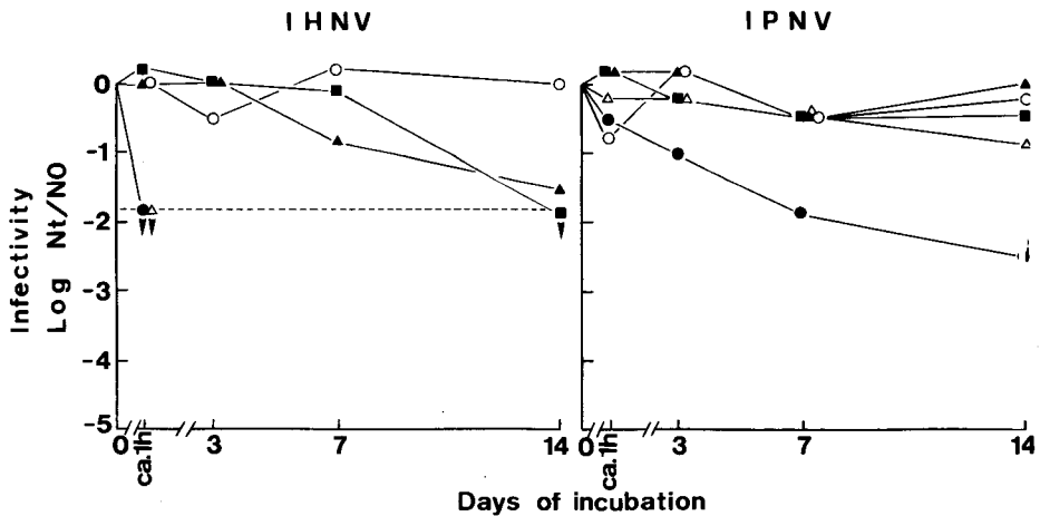
Fig. 1. Infectivities of fish pathogenic viruses in brackish water and water-sediment mixture samples from the estuary of the Moheji river in June, 1984. Symbols: ■, autoclaved; ▲, filtered; ●, untreated; △, water-sediment mixture; ○, control. Dotted line and arrows indicate detectable limits of viral titres and less than the limits respectively.
