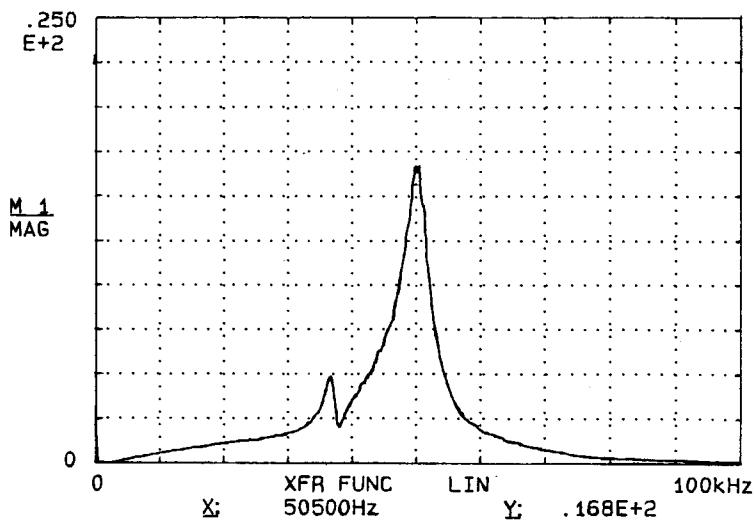
Fig. 5. Measured receiver's frequency transfer function of 50 kHz JRC-CFT-550 transducer.
