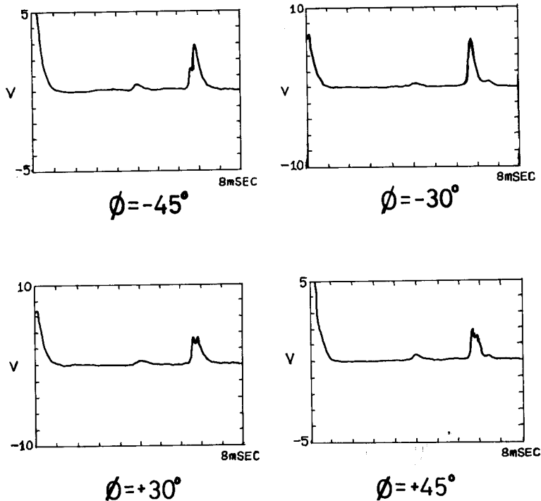
Fig. 8. Examples of the change of echo waveform in roll plane (near dorsal aspect) for 52.5 cm aka ika at 200 kHz.
