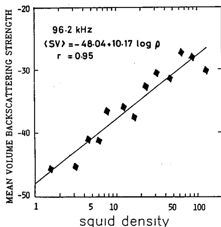
Fig. 9. The relationship between mean volume backscattering strength \langle SV \rangle (dB) and squid density \rho (squid/m 3 ) at 28.5 kHz and 96.2 kHz.
