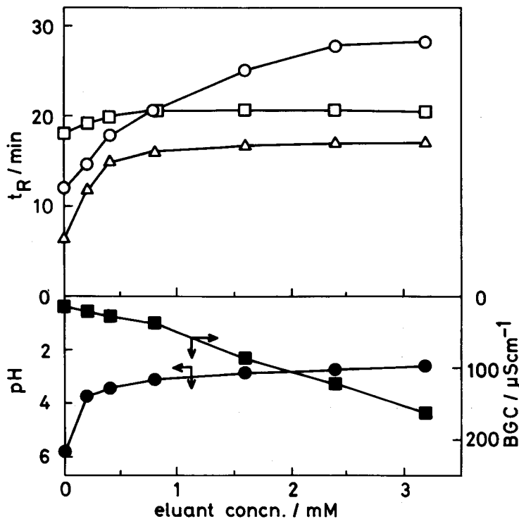
Fig. 2. Effect of eluant concentration on chromatographic performance.
