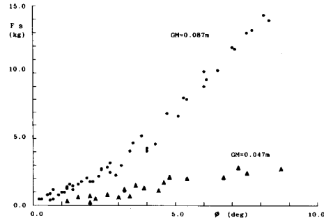
Fig. 13. Swaying force F_S .
