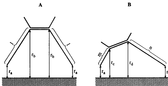
Fig. 4. System for locating cis monoethylenic fatty acid with respect to the stationary phase. A: In the case when the ethylene unit is at the center of the carbon chain, and B: when the ethylene unit is near the end of the carbon chain. r_a : van der Waals radius at the end of acyl carbon chain; r_b, r_c, r_d : van der Waals radiuses at the ethylene unit; l, m, n : carbon number (when it is m+n=21 ).
