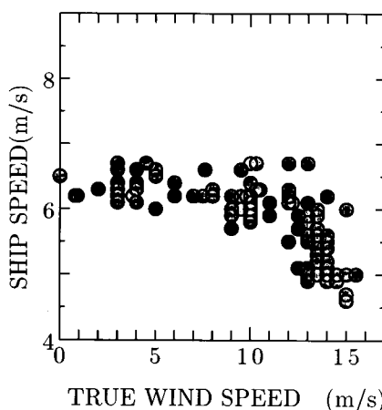
Fig. 6. Ship speed sea margin in head wind. Tidal current speed is within 0.9 knot.
