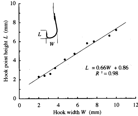
Fig. 2. Relationship between the hook width W and the hook point height L of sode hook. Marks, observed values; Line, calculated values.
