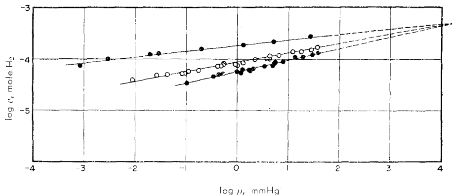
Fig. 1. Adsorption isotherm for hydrogen on a promoted iron catalyst at 20, 200 and 300°C. Ordinates represent adsorbed hydrogen per total catalyst 10.4 gm before reduction.
