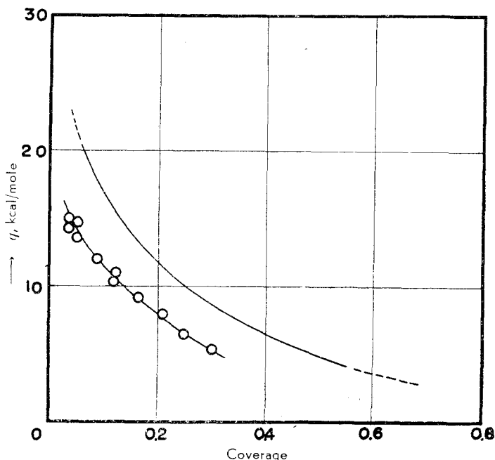
Fig. 2. The heat-coverage relationship. Hydrogen on a promoted iron catalyst.
