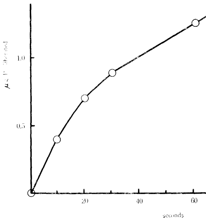
Fig. 4 Initial phase of insect myosin B ATPase. Conditions: pH 7.0, 37°C, (0.033 M-tris buffer), 0.6 M KCl, 5 mM MgCl 2 , 1.3 mg. protein per ml, total volume 1.5 ml.
