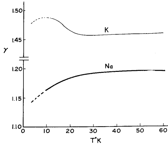
Fig. 7. Grüneisdn \gamma = \alpha V / \alpha C_V versus temperature for Na and K (theoretical).
