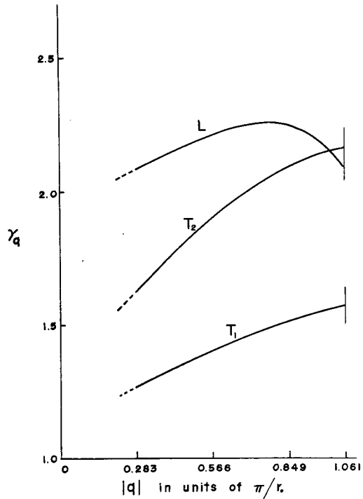
Fig. 12. The r_q versus wave number vector \mathbf{q} = \pi/r_0(\bar{q}, \bar{q}, 0) for Cu in the case of (b) E_0 = -3.7 eV.
