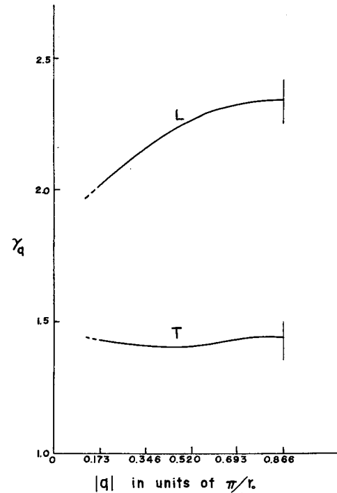
Fig. 13. The r_q versus wave number vector \mathbf{q} = \pi/r_0(\bar{q}, \bar{q}, \bar{q}) for Cu in the case of (b) E_0 = -3.7 eV.
