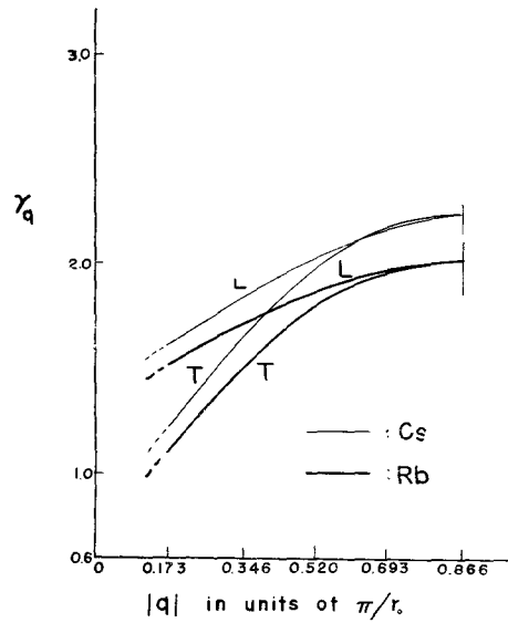
Fig. 6. The \gamma_q versus wave number vector \mathbf{q} = \pi/r_0 (\hat{q}, \hat{q}, \hat{q}) for Rb and Cs.
