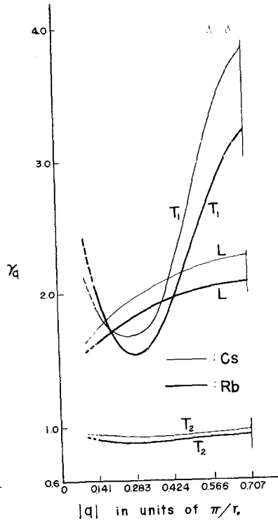
Fig. 5. The \gamma_q versus wave number vector \mathbf{q} = \pi/r_0 (\hat{q}, \hat{q}, 0) for Rb and Cs.
