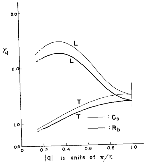
Fig. 4. The \gamma_q versus wave number vector \mathbf{q} = \pi/r_0 (\hat{q}, 0, 0) for Rb and Cs.
