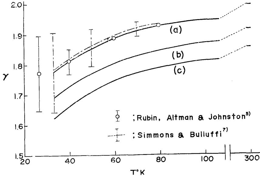
Fig. 14. Grüneisen \gamma = \alpha V / \alpha C_V versus temperature for Cu: (—) theoretical in the cases of (a) E_0 = -3.33 eV, (b) E_0 = -3.70 eV and (c) E_0 = -4.07 eV, respectively; - - - - SIMMONS and BULLUFFI (ref. 7); \circ Rubin, Altman and Johnston (ref. 5).
