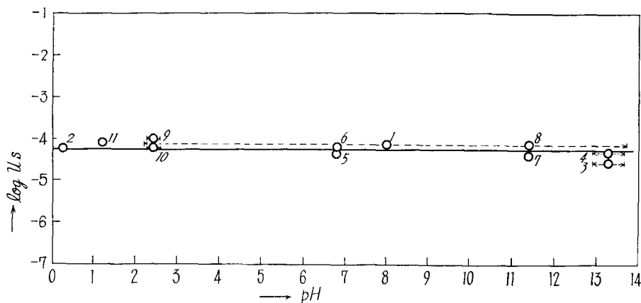
Fig. 2. Specific rate r/[\text{Cl}^-] \text{ min}^{-1} of chlorine transfer from solution to methylene chloride in one direction at 100^\circ\text{C} .
