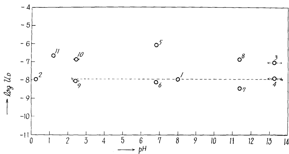
Fig. 1. Rate U_D \equiv r mol Cl/l. min of chlorine transfer from solution to methylene chloride in one direction at 100°C.
