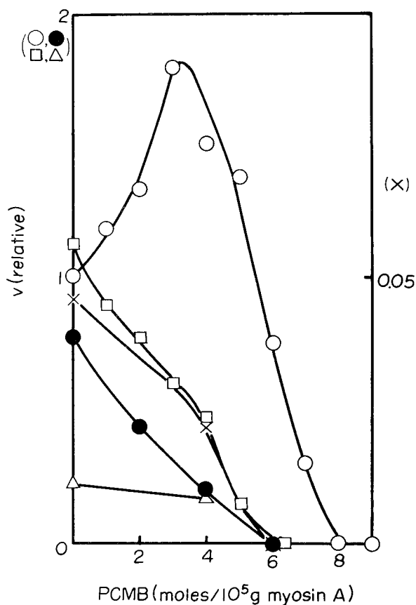
Fig. 6. Effect of PCMB on hydrolysis of ATP analogs. The concentrations of substrate and Ca^{2+} were 0.5 and 5 mM, respectively, except for TP, where both concentrations of the substrate and Ca^{2+} were 4 mM. PCMB was incubated with myosin A during 20 min. at 0° before start of the reaction. Experimental conditions: 0.5 M KCl, pH 7.0, 20°. Substrates: ATP (○), ITP (□), dimethyl ATP (△), BTP (●) and TP (×).
