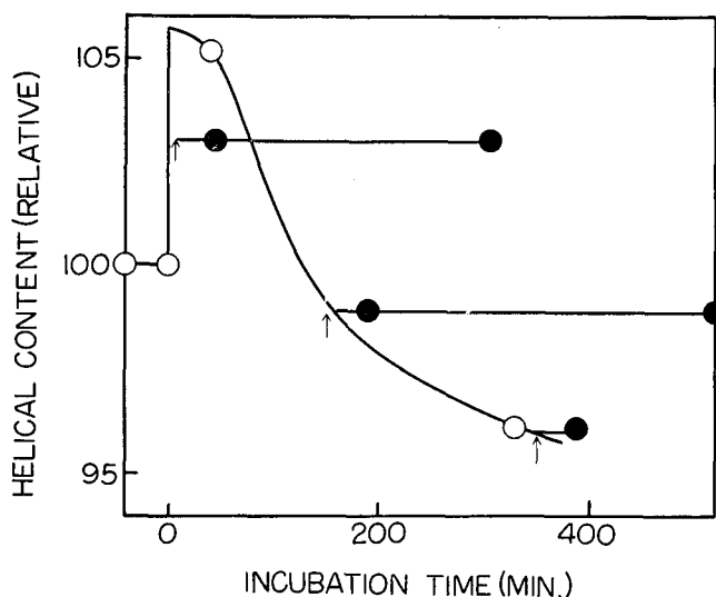
Fig. 13. Effect of PP_i on time-course of change in helical content in presence of dioxane. 0.6 M KCl, 6.14 mg myosin A/ml. pH 7.0, 20°. 8% purified dioxane was added at time 0. ○, in absence of PP_i ; ●, in presence of 1 mM Mg^{2+}\text{-PP}_i . Arrow indicates addition of Mg^{2+}\text{-PP}_i .
