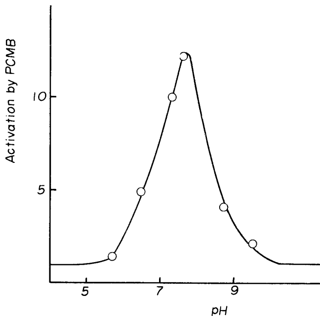
Fig. 4. Dependence on pH of maximum value of degree of activation by PCMB. Binding of PCMB: 0.8 M KCl, pH 6.7, 20°, 30 minutes. Assay of ATPase: 0.6 M KCl, 7 mM Ca 2+ , 1 mM ATP, 20°.
