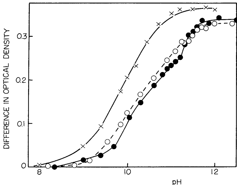
Fig. 14. Spectrophotometric titration of myosin A. 0.5 M KCl, 50 mM piperidine buffer, 1 mg myosin A/ml, 25°. O, control; x, 1.2 M urea-5 M guanidine HCl. The line is theoretical one for dissociation of a single group whose pK is 9.85. ●, 0.5 mM Mg^{2+} - PP_i .
