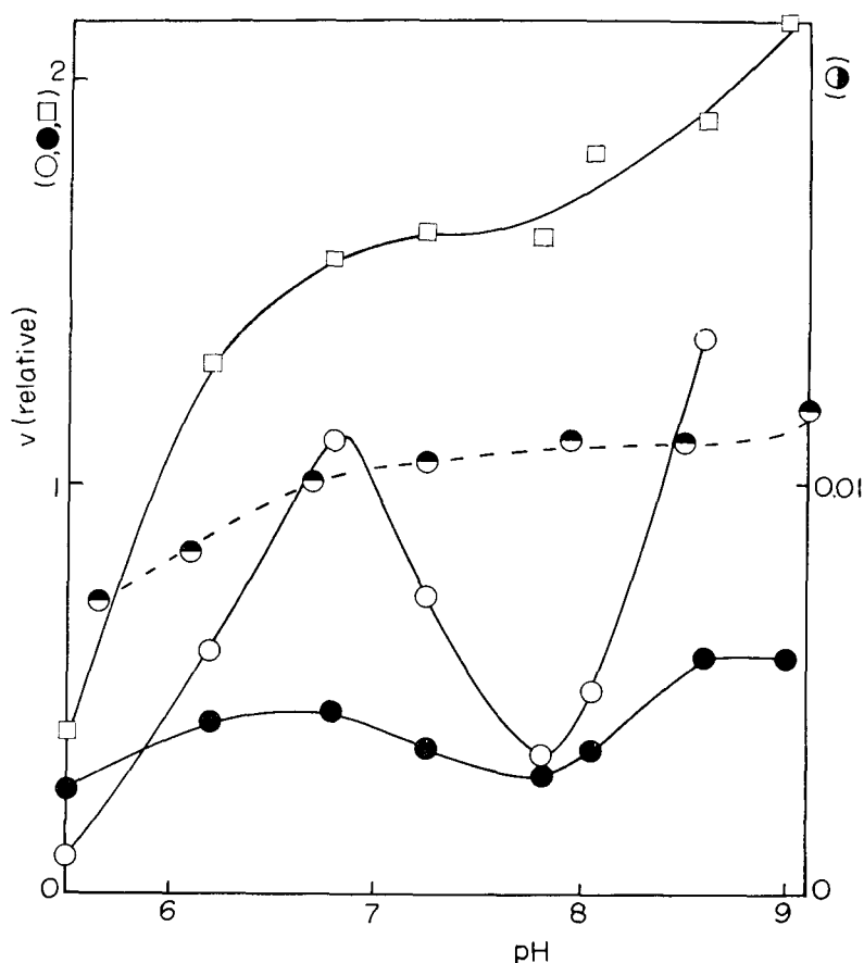
Fig. 7. pH dependence of myosin A NTPase. Tris-maleate buffer (25 mM) was used in the range of pH from 5.5 to 7.8 and Tris-HCl buffer (25 mM) in the range of pH from 7.8 to 9.1. The concentrations of the substrate and \text{Ca}^{2+} were 0.5 and 5 mM, respectively. Experimental conditions: 0.5 M KCl, 20°. Substrates: ATP (○), ITP (□), BTP (●) and RTP (◐).
