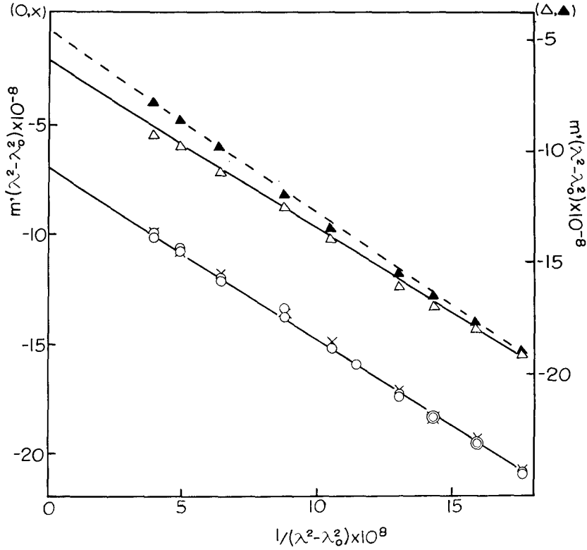
Fig. 10. MOFFITT-YANG plot of dispersion data in presence of Mg^{2+} -ADP and Mg^{2+} -ATP. 0.6 M KCl, 20 mM Mg^{2+} , 3.81 mg myosin A/ml, pH 7.0, 13°. O, control; ×, 3 mM ADP. △, control; ▲, 3 mM ATP.
