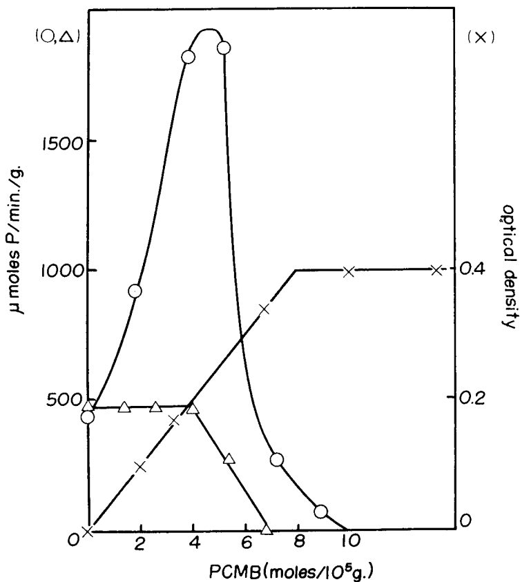
Fig. 5. Effect of PCMB on ATPase of TNP-myosin A. 0.6 M KCl, 7 mM Ca 2+ , 1 mM ATP, pH 7.0, 20°. ○, original myosin A; △, 1.35 mole of TBS/2.1 × 10 5 g of myosin A; ×, spectrophotometric titration of SH group of TNP-myosin A with PCMB.
