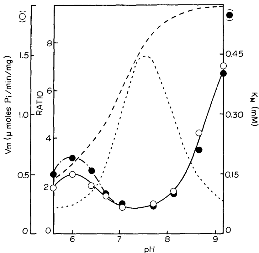
Fig. 2. Effect of pH on V_m and K_M of myosin A ATPase. Reaction mixture: 0.6 M KCl, 7 mM Ca^{2+} and 0.088 mg myosin A/ml. 20°. \circ , V_m ; \bullet , K_M . Broken line is pH-dependence of k_2 . Dotted line is the theoretical curve of pH-dependence of 1+K .
