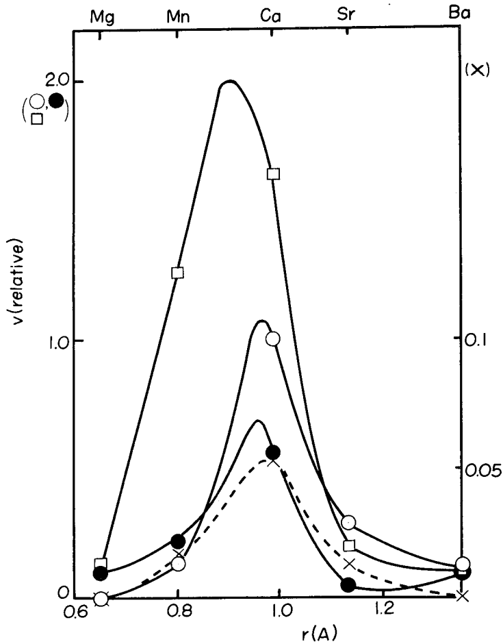
Fig. 1. Effect of divalent cation on myosin A NTPase. The ordinate indicates relative activity, ATPase for the same preparation of myosin A in presence of 5 mM \text{Ca}^{2+} being defined as 1. The abscissa indicates ionic radius of added divalent cation. The concentrations of substrate and divalent cation were 0.5 and 5 mM, respectively, except for TP, where both concentration of the substrate and divalent cation were 4 mM. Experimental conditions: 0.5 M KCl, pH 7.0, 20°. Substrates: ATP (○), ITP (□), BTP (●) and TP (×).
