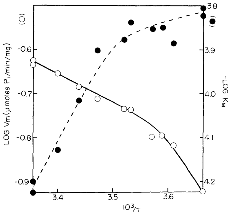
Fig. 3. Effect of temperature on V_m and K_M of myosin A ATPase. Reaction mixture: 0.6 M KCl, 7 mM C^{2+} , 25 mM Tris and 0.11 mg myosin A/ml. pH 7.05. O, log V_m ; ●, -\log K_M .
