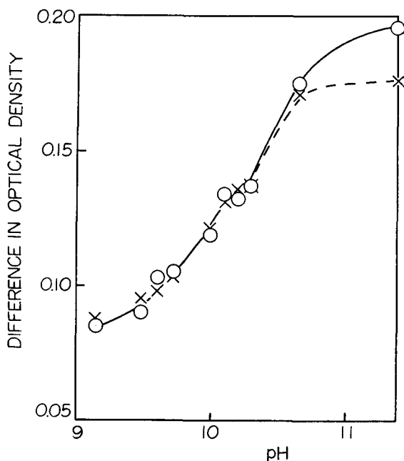
Fig. 15. Effect of ATP on nitroprusside color development of myosin A. Light pass, 1 cm. O, 1.72 mg myosin A/ml. plus 45 mM nitroprusside, 0.3 M KCl at 0°. X, 1.72 mg myosin A/ml. plus 2 mM ATP, 5 mM Mg^{2+} and 45 mM nitroprusside, 0.3 M KCl at 0°.
