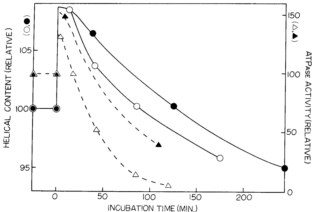
Fig. 12. Time-courses of changes in helical content (O, ●) and ATPase activity (△, ▲) after addition of dioxane. 0.6 M KCl, pH 7.0, 20°. Helical content was estimated from b_0 term and ATPase activity measured in 7 mM Ca 2+ , 0.5 mM ATP and 10 mM Tris-maleate buffer. Helical content: O, 10 volume % dioxane, 4.65 mg myosin A/ml; ●, 8 volume % purified dioxane, 3.62 mg myosin A/ml. ATPase activity: △, 10 volume % dioxane, 0.2 mg myosin A/ml; ▲, 8 volume % purified dioxane, 0.2 mg myosin A/ml.
