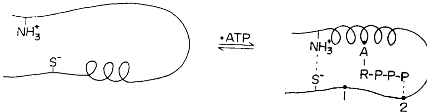
Fig. 11. A formation of active site by conformation change and salt-bridge.
