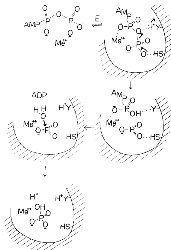
Fig. 8. A tentative scheme of cleavage of pyrophosphate bond catalyzed by myosin A.
