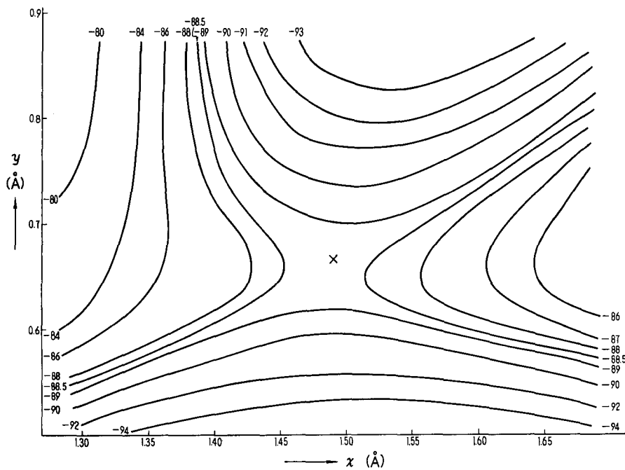
Fig. 9. \epsilon^*(x, y) calculated by Eq. (13) for seat afforded by a pair of 2.883 \text{ \AA} spaced metal atoms on (111)-lattice plane. Energy is referred to that of the state where four atoms are at rest infinitely apart from each other. X indicates the saddle point.
