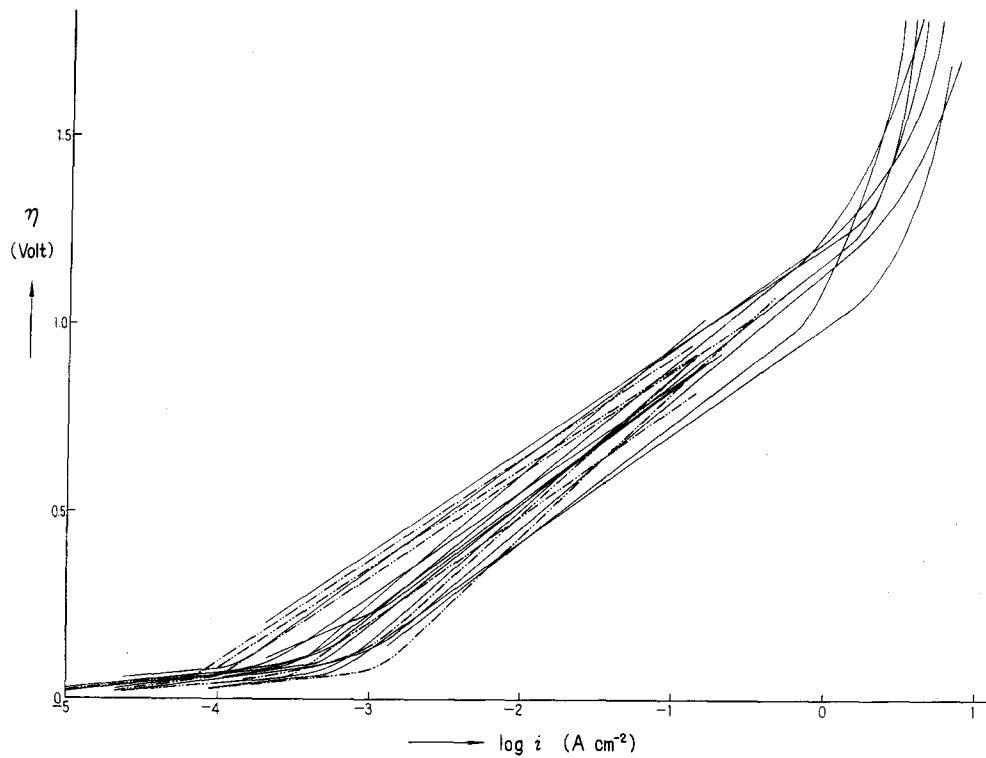
Fig. 6. Relationship between the overvoltage, \eta , and \log i on electrode (C) at 21 \pm 2^\circ C . — : 1.11 \pm 0.01 N NaOH ..... : 0.26 \pm 0.01 N NaOH
