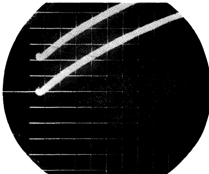
Plate 11. The potential-time variation after switching on a polarizing current on Pt in aqueous 0.1 N Na 2 SO 4 , pH 8.3, i = 1 \cdot 10^{-3} mp., 1 mv/Div, 10 \mu sec/Div.
