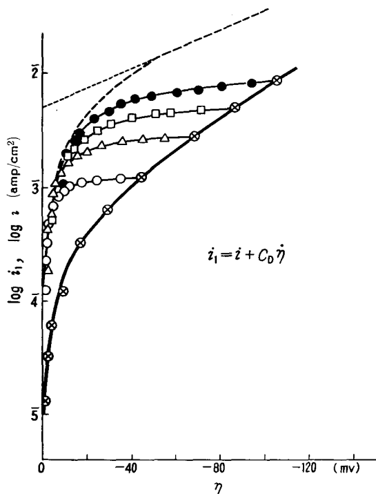
Fig. 15. The relation between \log i_1 vs. \eta in the build up processes, and \log i vs. \eta in steady states in \text{NaOH}_{\text{aq}} , pH 13.0; the polarizing current (○) 1.2 \cdot 10^{-3} amp/cm ^2 , (△) 2.7 \cdot 10^{-3} amp/cm ^2 , (□) 4.8 \cdot 10^{-3} amp/cm ^2 , (●) 8.3 \cdot 10^{-3} amp/cm ^2 ; (⊗) denotes \log i vs. \eta in steady states.
