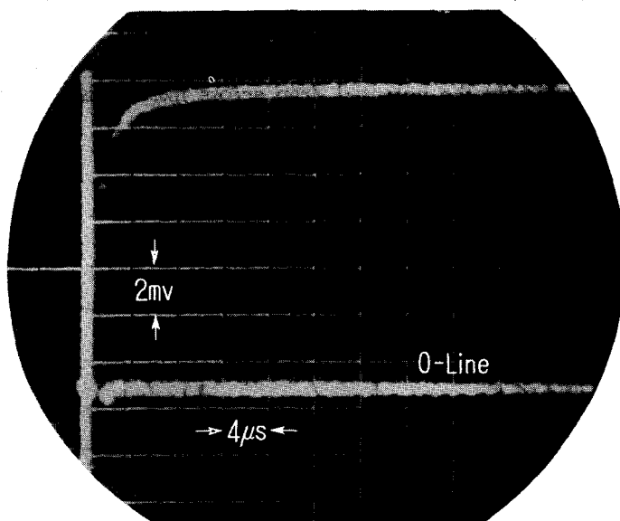
Plate 1. The current-time variation after switching on. The ordinate shows potential drop across R_2 ( 100 \Omega ), 2 \text{ mv/Division} ; the abscissa time after switching on, 4 \mu\text{sec/Div.} ; solution 0.1 \text{ N Na}_2\text{SO}_{4,\text{aq}} , pH 8.3.
