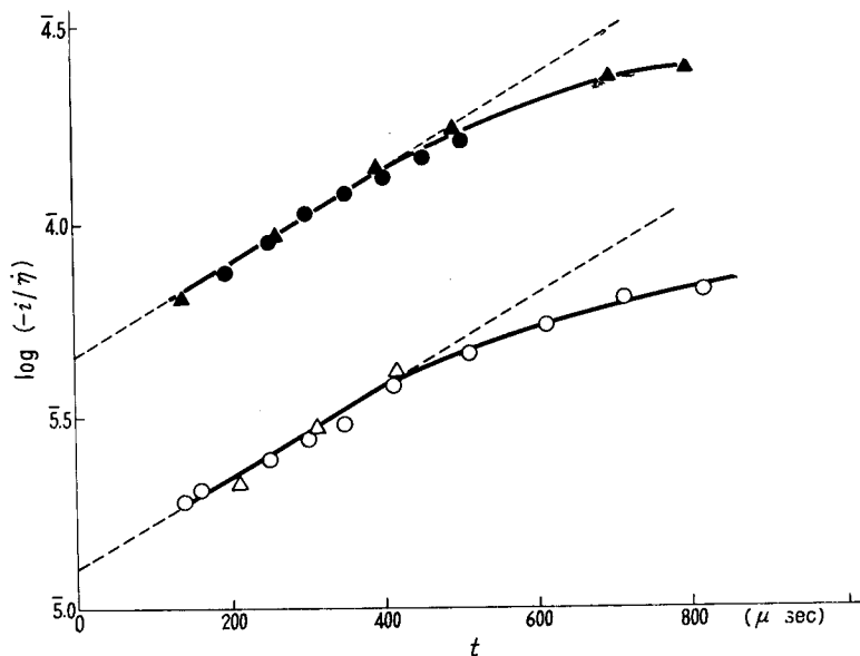
Fig. 11. The relation between \log(-i/\eta) and time in the build up processes in \text{NaOH}_{aq} , pH 11.9, the electrodes are the same as in Fig. 10; the currents (O) 2.23 \cdot 10^{-4} amp, ( \Delta ) 4.06 \cdot 10^{-4} amp; (●) 4.06 \cdot 10^{-4} amp; C^D = 13 and 44 \mu\text{F} respectively and \tau_1 = 326 \mu\text{sec} .
