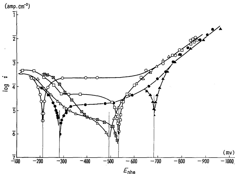
Fig. 10. \log i vs. E_{nhe} in steady states on Pt; (O) in 0.1 N \text{Na}_2\text{SO}_4 , pH 3.53; ( \Delta ) in 0.01 N \text{Na}_2\text{SO}_4 , pH 8.2; ( \square ) and ( \boxtimes ) in 0.1 N \text{Na}_2\text{SO}_4 , pH 8.9, respectively in vigorous stirring by hydrogen bubbles and weak one; ( \bullet ) in 1 N \text{Na}_2\text{SO}_4 , pH 4.7; ( \blacktriangle ) in 1 N \text{Na}_2\text{SO}_4 , pH 11.38.
