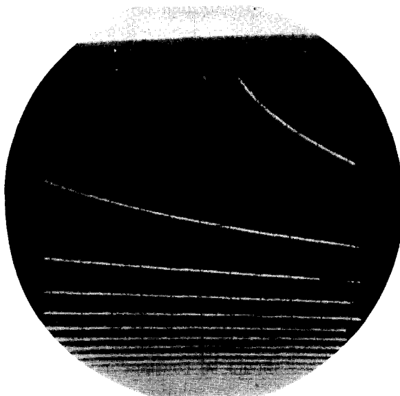
Plate 1. The potential-time variation after switching off a polarizing current on an evaporated platinum film in \text{NaOH}_{\text{aq}} , pH 13.3; i = 2.0 \cdot 10^{-3} amp · cm ^{-2} , the ordinate 20 mv/Div, the abscissa 100 \mu sec/Div.
