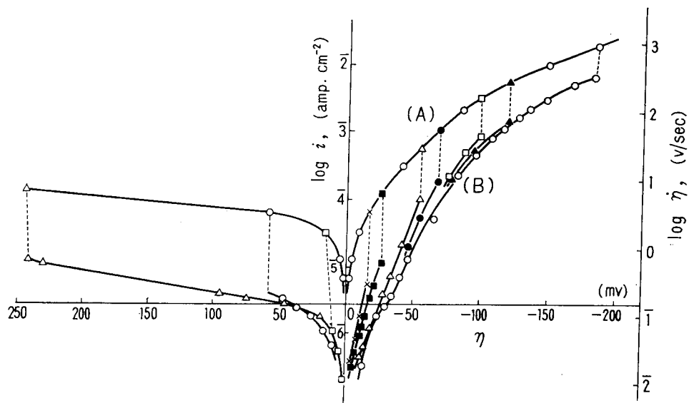
Fig. 4. The \log i vs. \eta in steady states, and \log \dot{\gamma} vs. \eta in the decay processes on a platinum film in \text{NaOH}_{\text{aq}} , pH 13.10.
