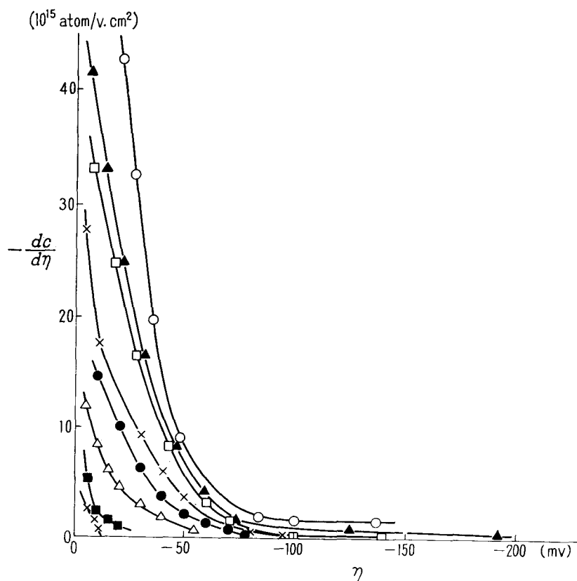
Fig. 2. The -dc/d\eta vs. \eta calculated from Fig. 1. The signs correspond respectively to those in Fig. 1.
