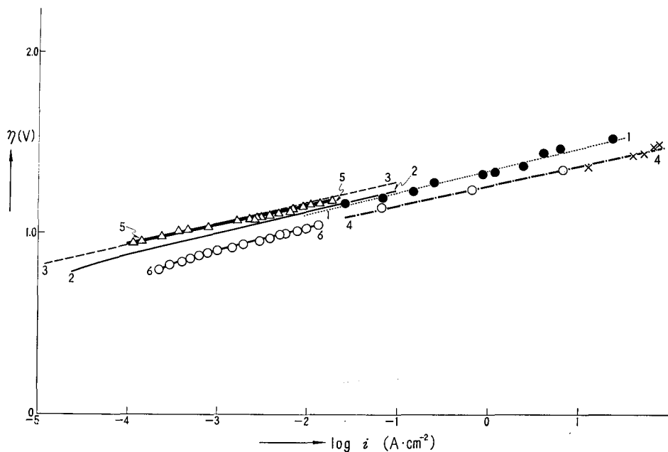
Fig. 4. Comparison of the present results with others. 1; Present result (1N H 2 SO 4 ), 2; DE BETHUNE 16 ) (1.005N HCl, 25±0.02°C), 3; POST and HISKEY 17 ) (0.1N HCl, 21±0.1°C), 4; BOCKRIS and AZZAM 18 ) (5N HCl, 25°C), 5; BUTLER and MAKRIDES 19 ) (0.1 N HClO 4 , 25°C), 6; CONWAY and SALOMON 20 ) (1N HCl-CH 3 OH, 27°C).
