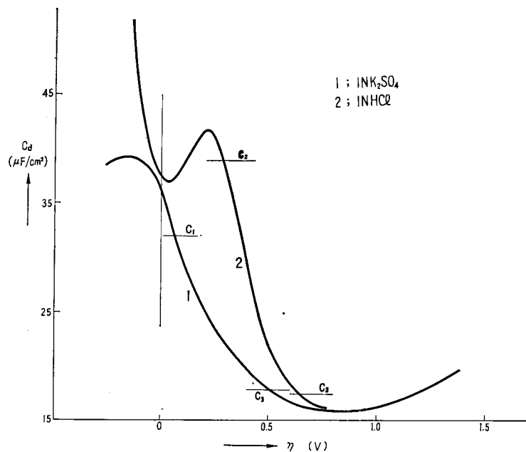
Fig. 2. C_d vs \eta curve reported in 1\text{N K}_2\text{SO}_4 10) and 1\text{N HCl} 15) . Horizontal lines represent mean values of C_{d1} , C_{d2} and C_{d3} in Table 2 and length indicates potential range at which respective values of C_d 's are observed.
