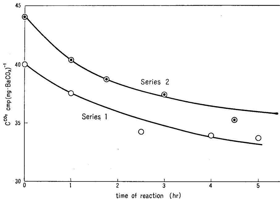
Fig. 5. Variation of C^{CO_2} with time of reaction.
