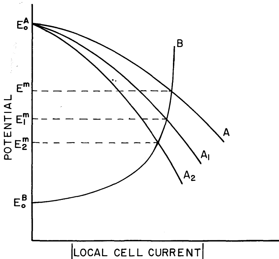
Fig. 4. A sketch of the local cell polarization curves for the O_2/H_2O reaction, curve A, and the metal/metal-oxygen reaction, curve B. Curves A_1 and A_2 represent the polarization on electrodes with increasing Rh content with corresponding mixed potentials, E_1^m , and E_2^m . E_o^A and E_o^B are the equilibrium potentials for the O_2/H_2O reaction (1,229 mV) and the metal/metal-oxygen reaction ( \sim 880 mV).
