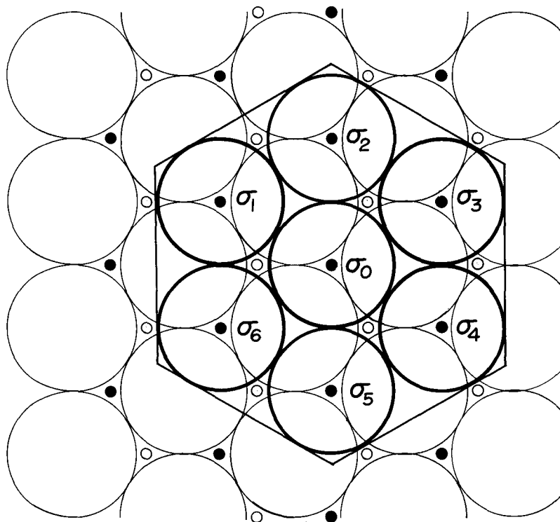
Fig. 1. Sites of adsorption on the surface of bulk liquid. ○ signifies an orthograph of a molecule composing the surface of bulk liquid, and ○ that of molecule adsorbed on the surface. ● denotes adsorption sites of a class and ○ that of the other, either of them being exclusively occupied by molecules closest packed in a layer; the set of sites, \sigma_0, \dots, \sigma_5 , and \sigma_6 , circumscribed by a regular hexagon is signified by \Sigma .
